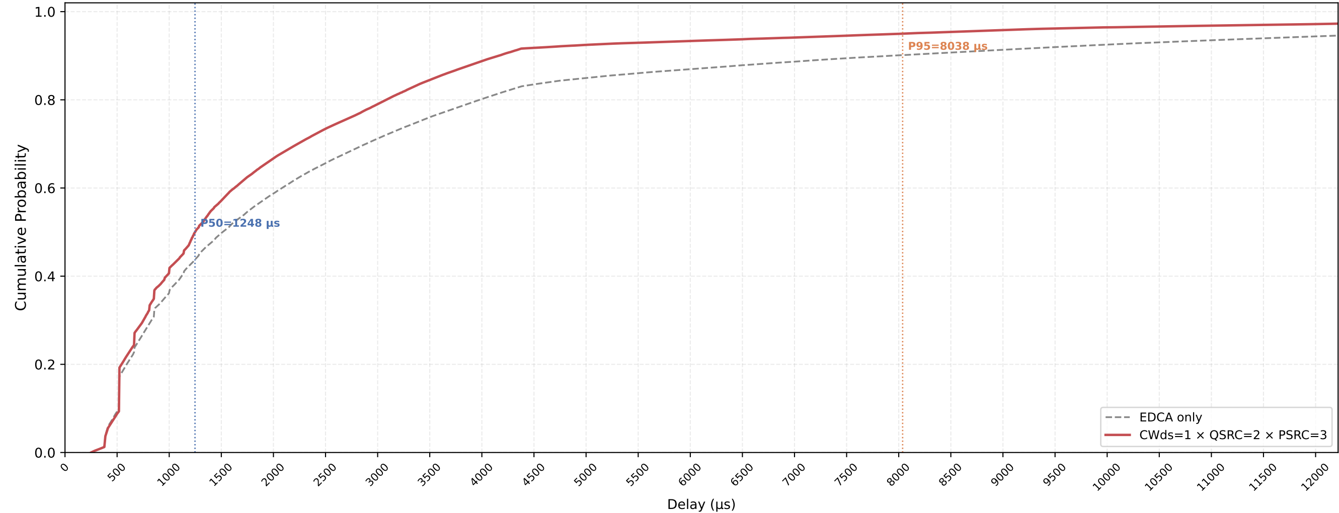
P-EDCA STA VO Delay CDF — CWds=1 × QSRC=2 × PSRC=3 nSta=30, nPedca=15, 1Mbps, avg of 10 runs
