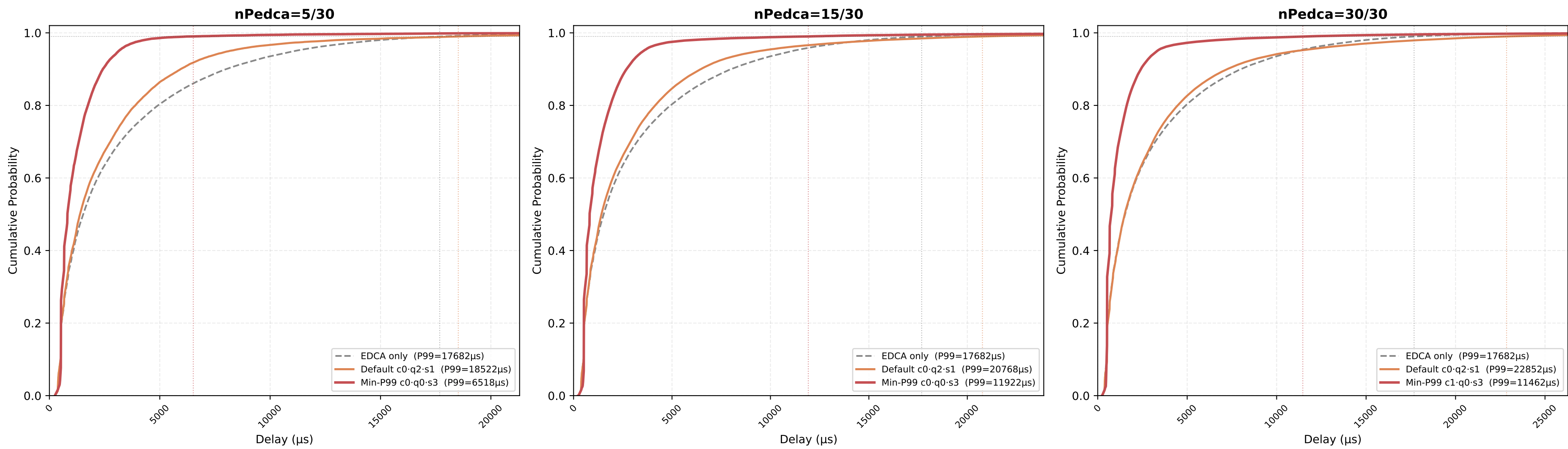
P-EDCA STAs — Min-P99 vs Default (c0·q2·s1) vsEDCA-only | nSta=30, 1Mbps, 10 runs avg
