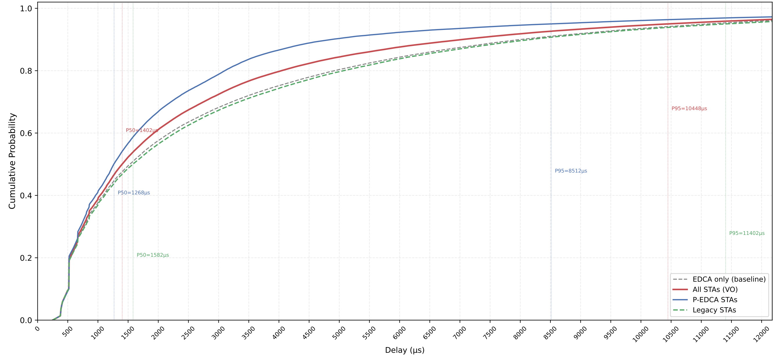
VO Delay CDF — P-EDCA / Legacy / All | CWds=0 × QSRC=1 × PSRC=1 nSta=30, nPedca=15/30, 1Mbps, avg of 10 runs
