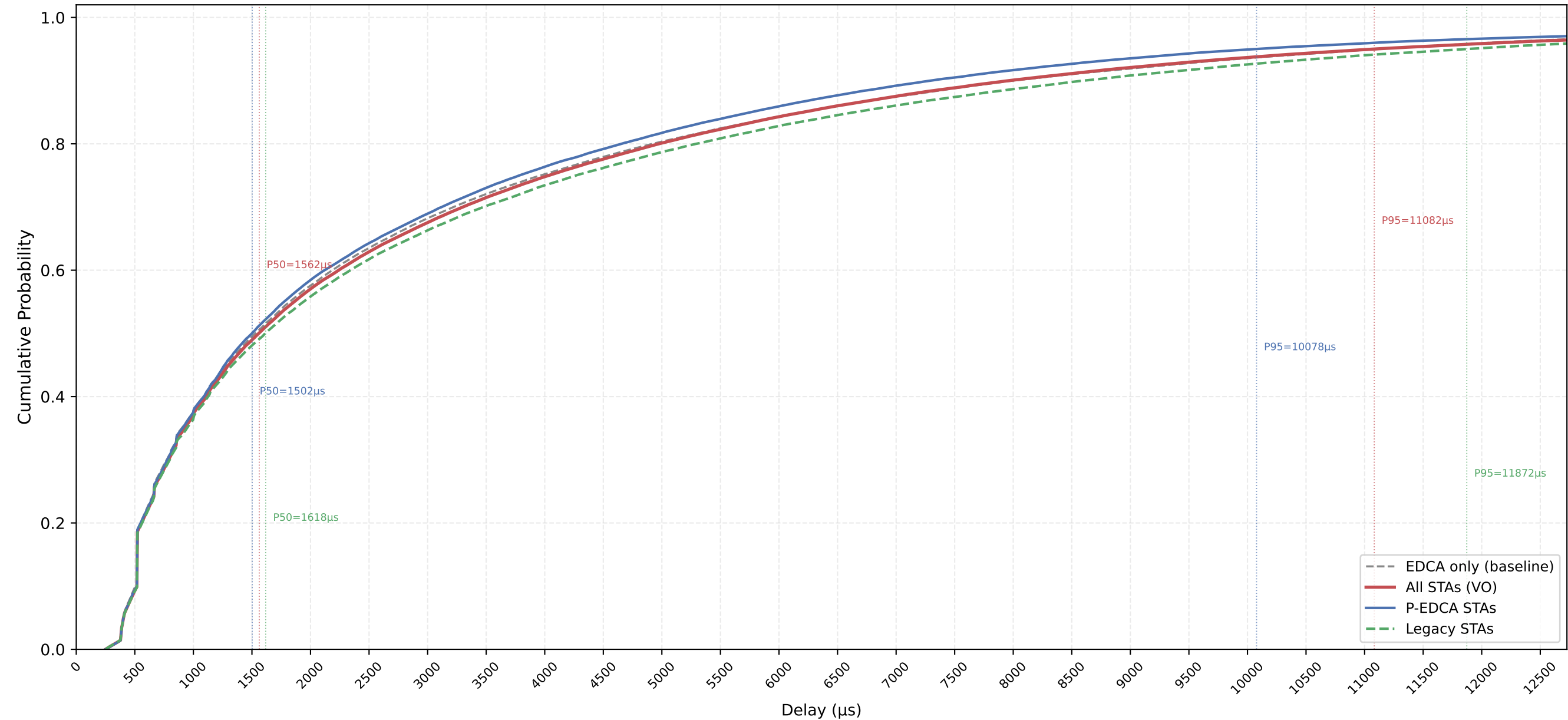
VO Delay CDF — P-EDCA / Legacy / All | CWds=0 × QSRC=3 × PSRC=1 nSta=30, nPedca=15/30, 1Mbps, avg of 10 runs
