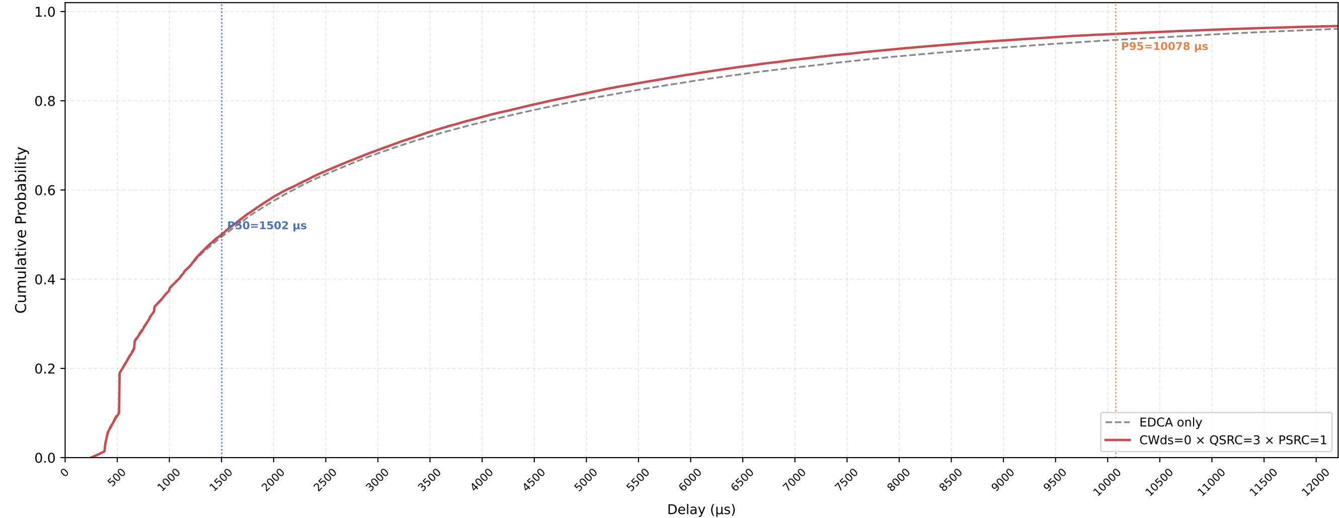
P-EDCA STA VO Delay CDF — CWds=0 × QSRC=3 × PSRC=1 nSta=30, nPedca=15, 1Mbps, avg of 10 runs
