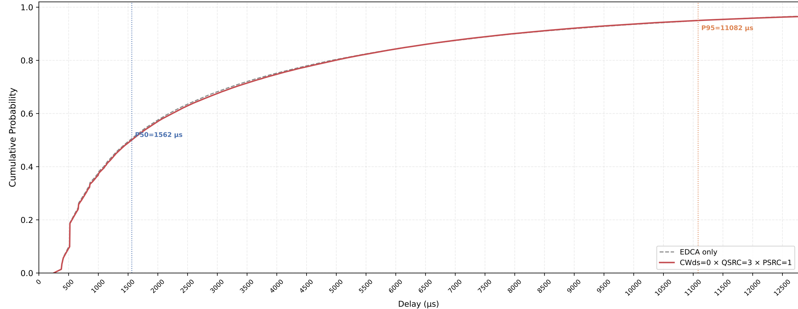
VO (all STAs) Delay CDF — CWds=0 × QSRC=3 × PSRC=1 nSta=30, nPedca=15, 1Mbps, avg of 10 runs
