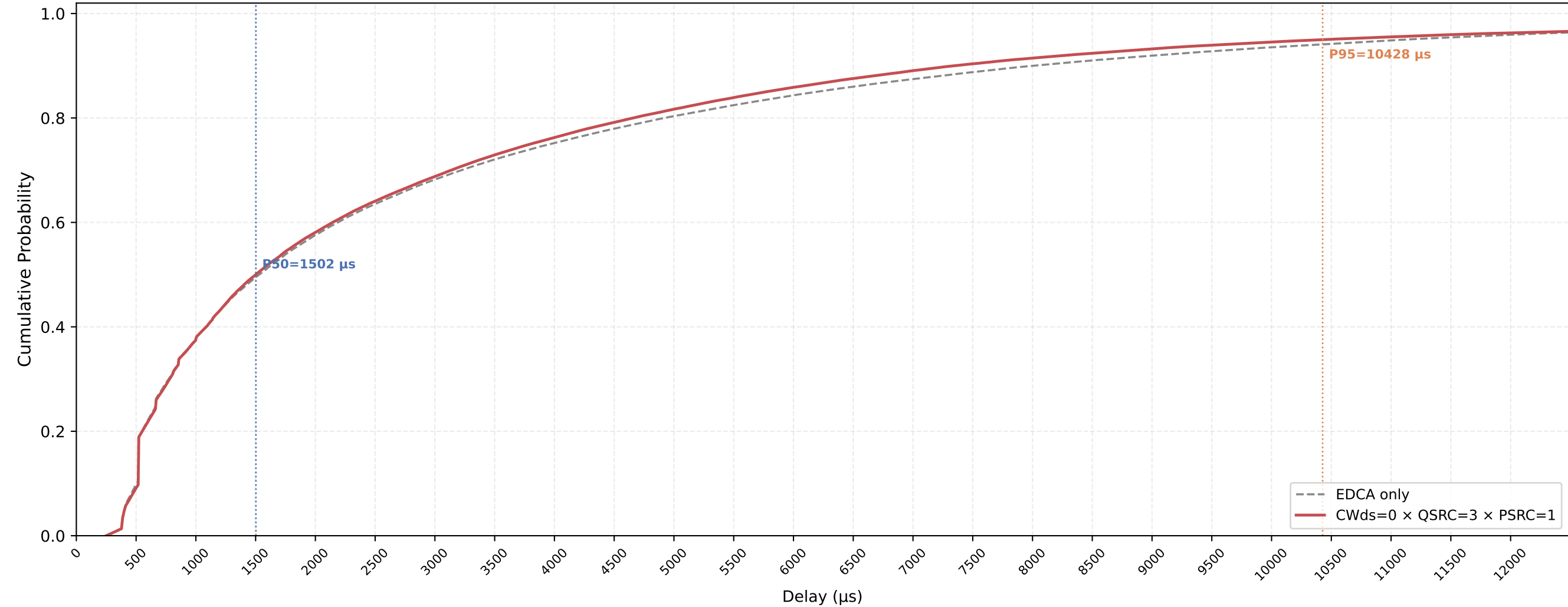
VO (all STAs) Delay CDF — CWds=0 × QSRC=3 × PSRC=1 nSta=30, nPedca=30, 1Mbps, avg of 10 runs
