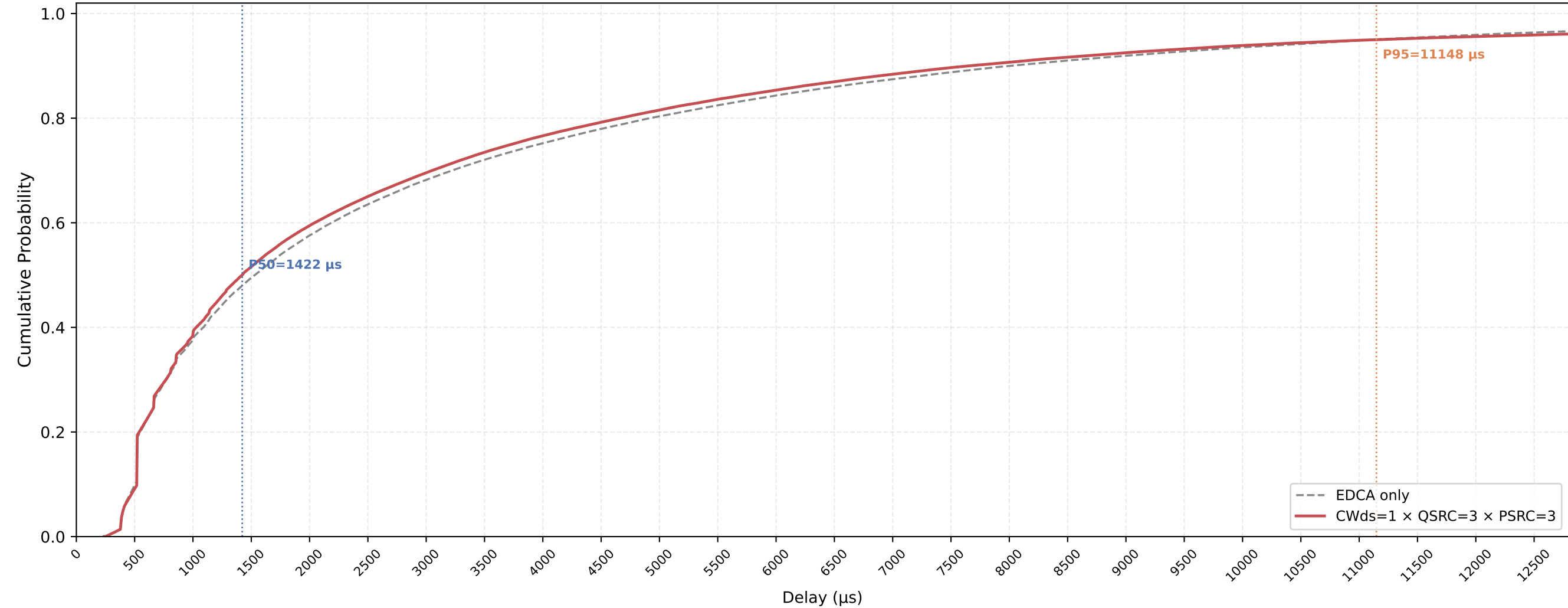
P-EDCA STA VO Delay CDF — CWds=1 × QSRC=3 × PSRC=3 nSta=30, nPedca=30, 1Mbps, avg of 10 runs
