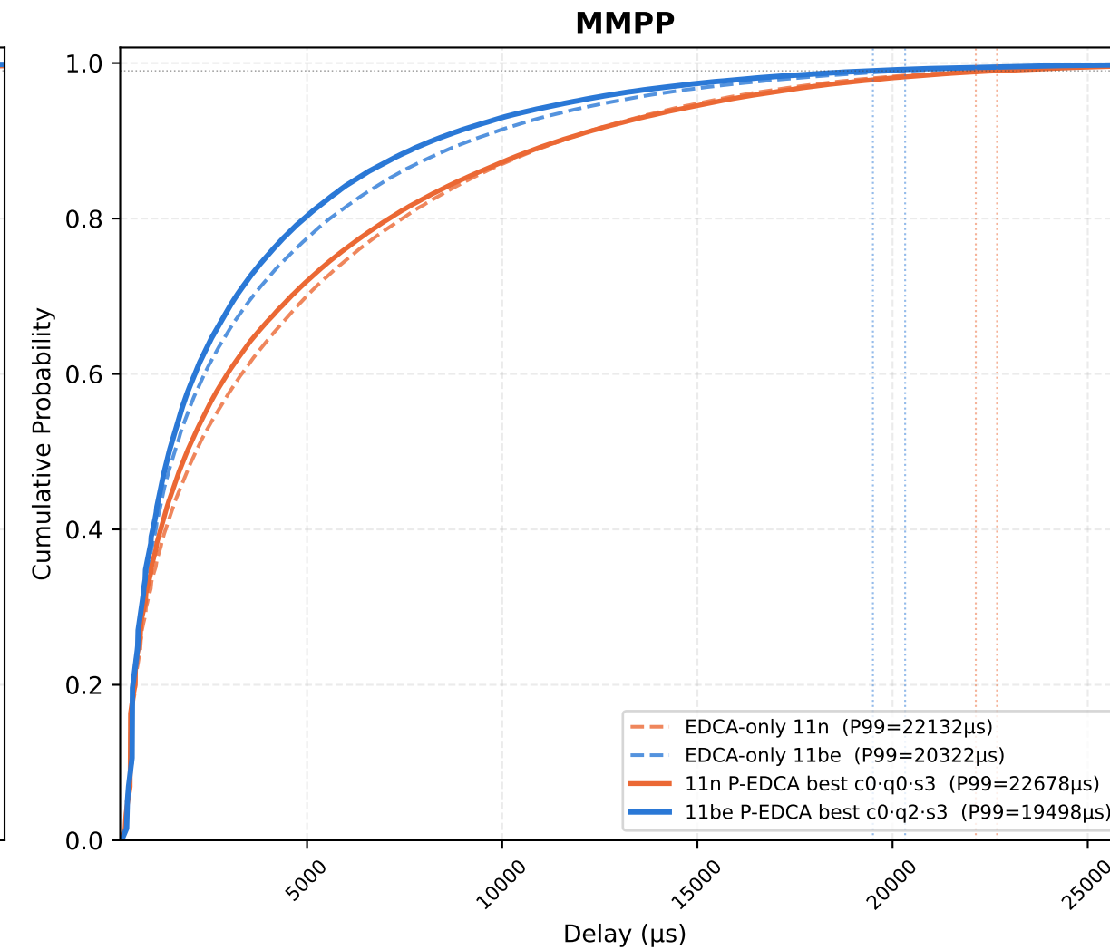
All STAs — EDCA-only (11n / 11be) vs Best-param P-EDCA (11n / 11be) | nPedca=5/30, nSta=30, 1Mbps, 10 runs avg
