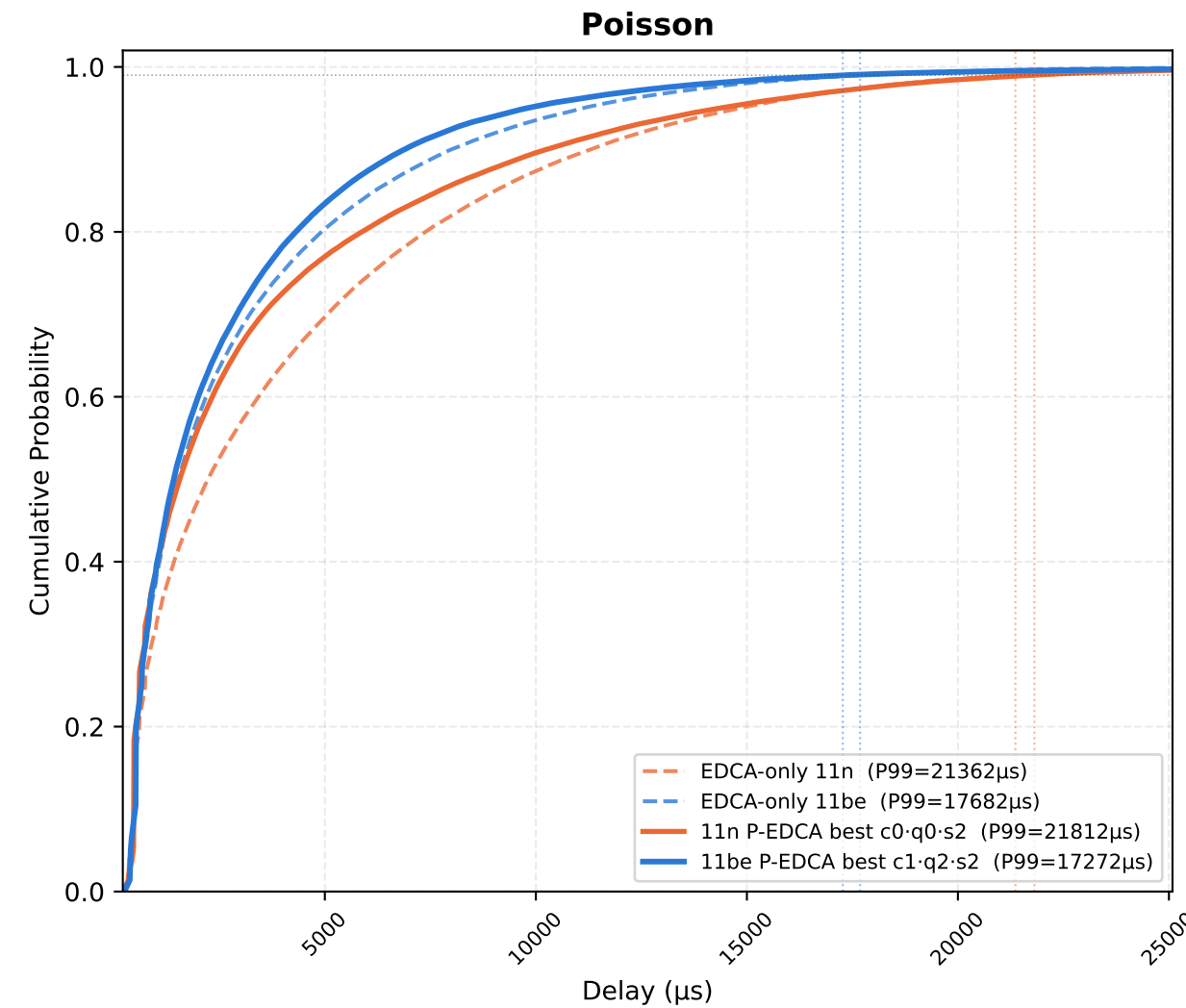
All STAs — EDCA-only (11n / 11be) vs Best-param P-EDCA (11n / 11be) | nPedca=15/30, nSta=30, 1Mbps, 10 runs avg
