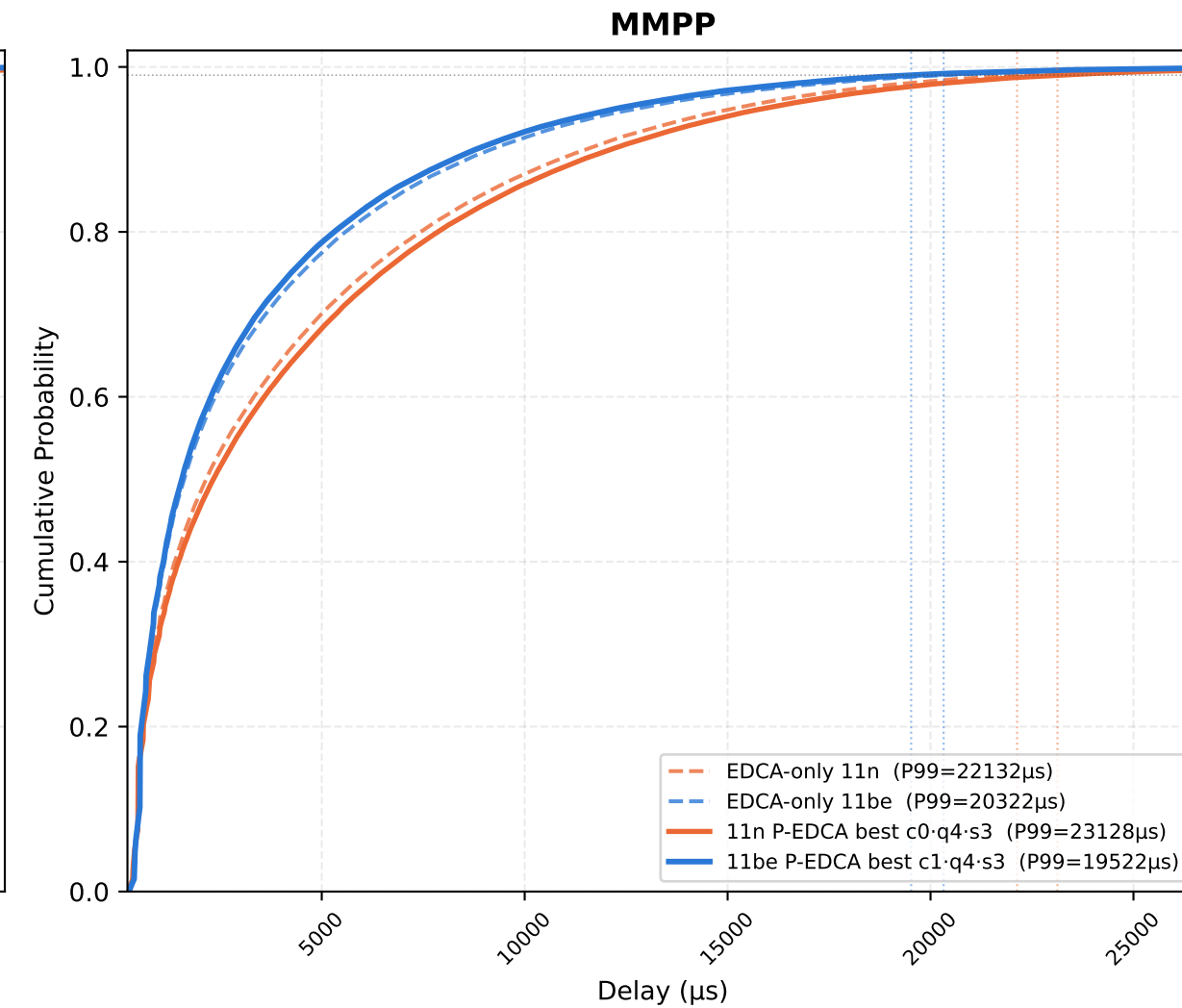
Legacy STAs — EDCA-only (11n / 11be) vs Best-param P-EDCA (11n / 11be) | nPedca=5/30, nSta=30, 1Mbps, 10 runs avg
