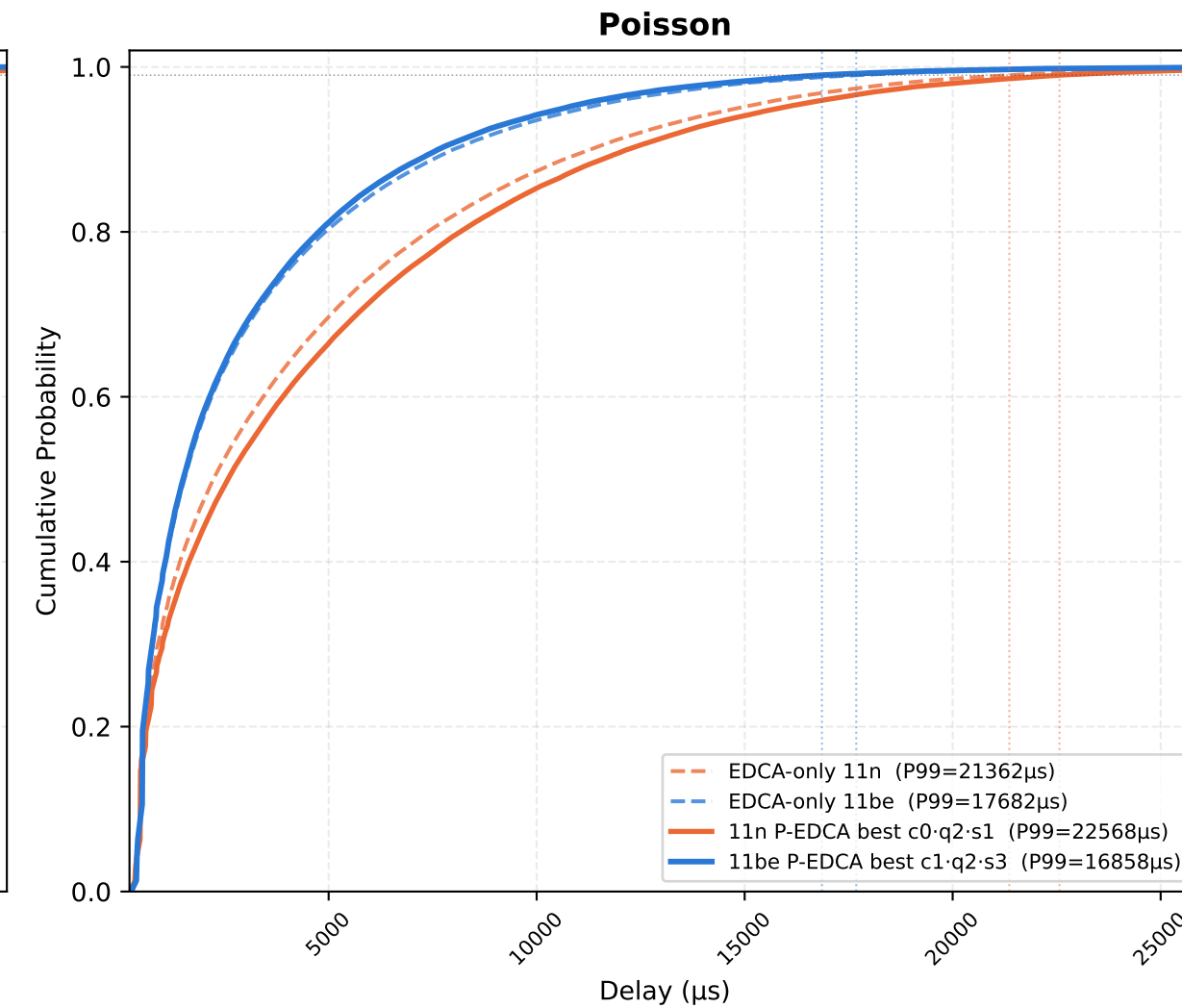
Legacy STAs — EDCA-only (11n / 11be) vs Best-param P-EDCA (11n / 11be) | nPedca=15/30, nSta=30, 1Mbps, 10 runs avg
