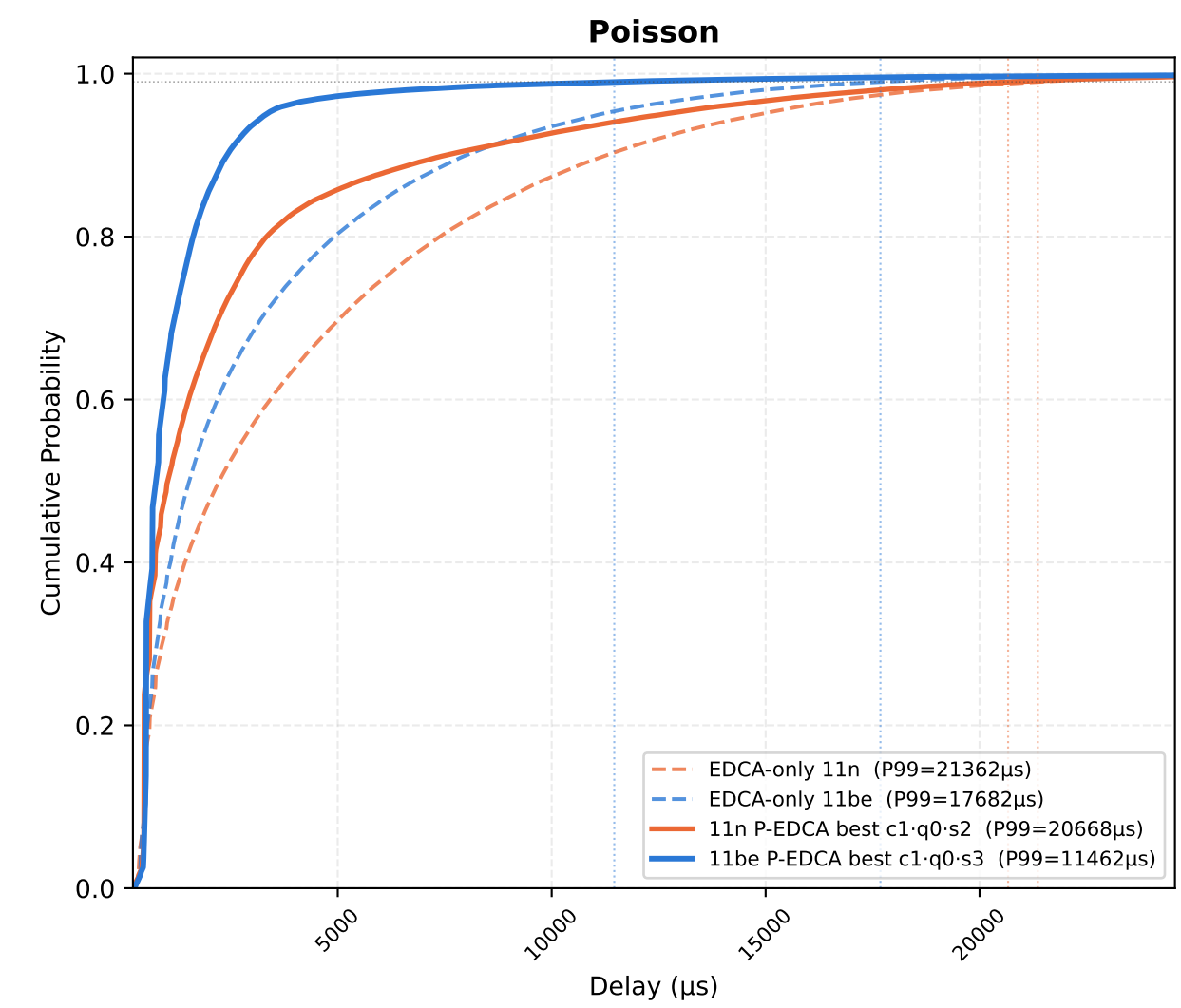
P-EDCA STAs — EDCA-only (11n / 11be) vs Best-param P-EDCA (11n / 11be) | nPedca=30/30, nSta=30, 1Mbps, 10 runs avg
