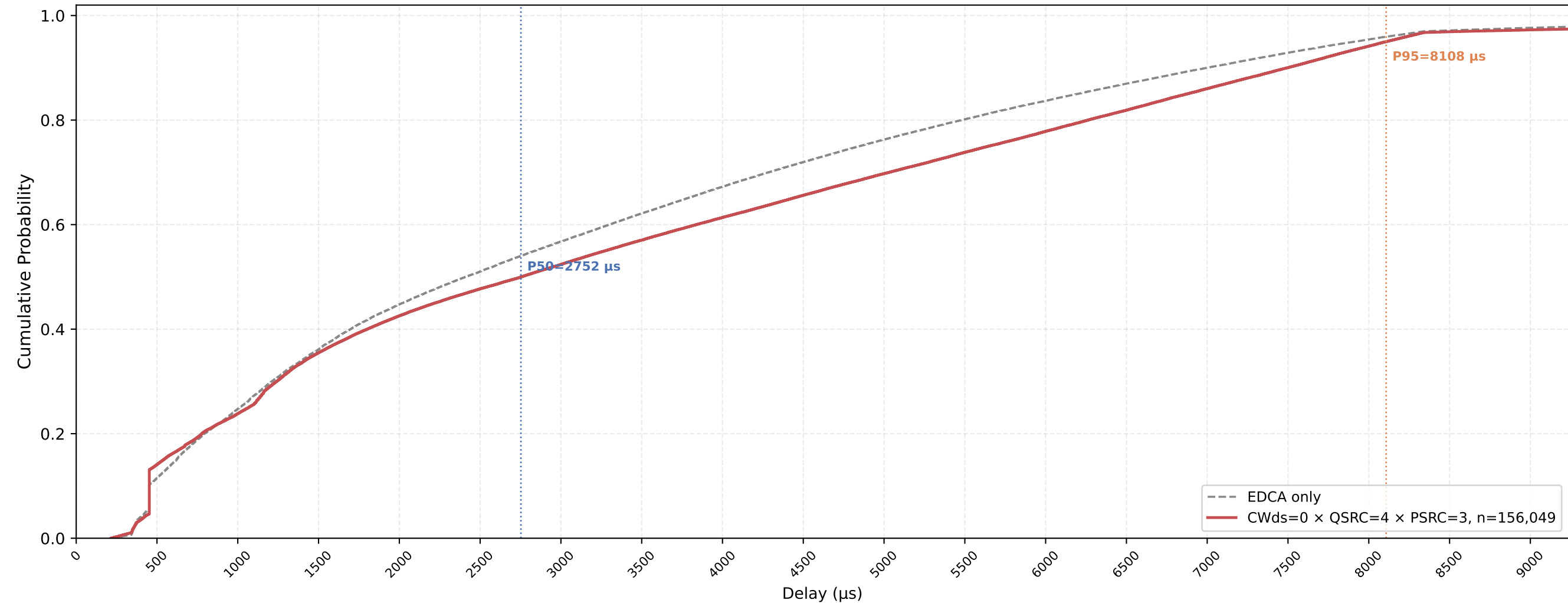
VO (all STAs) Delay CDF — CWds=0 × QSRC=4 × PSRC=3 nSta=30, nPedca=30, 1Mbps, avg of 10 runs
