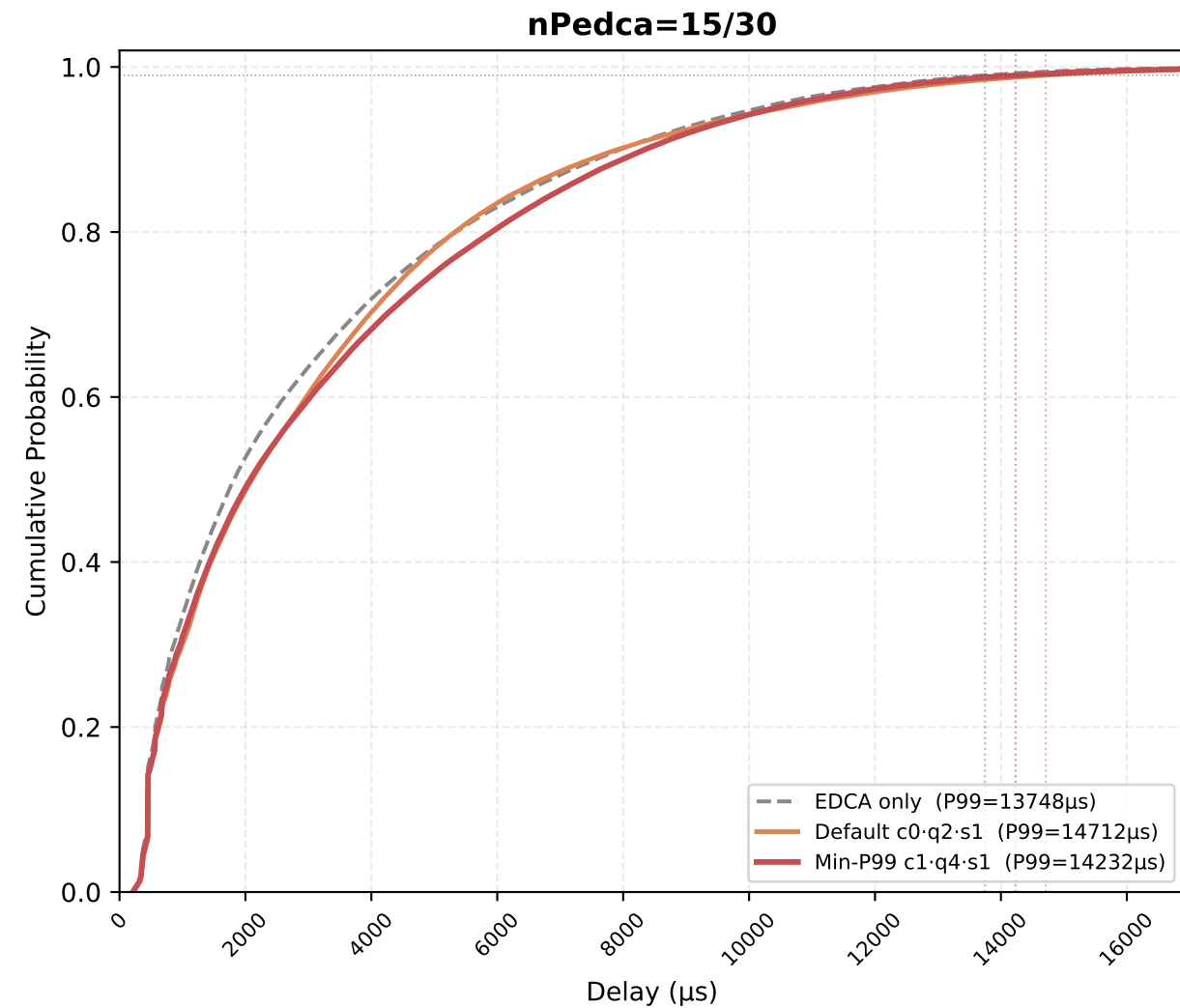
All STAs — Min-P99 vs Default (c0·q2·s1) vs EDCA-only | nSta=30, 1Mbps, 10 runs avg
