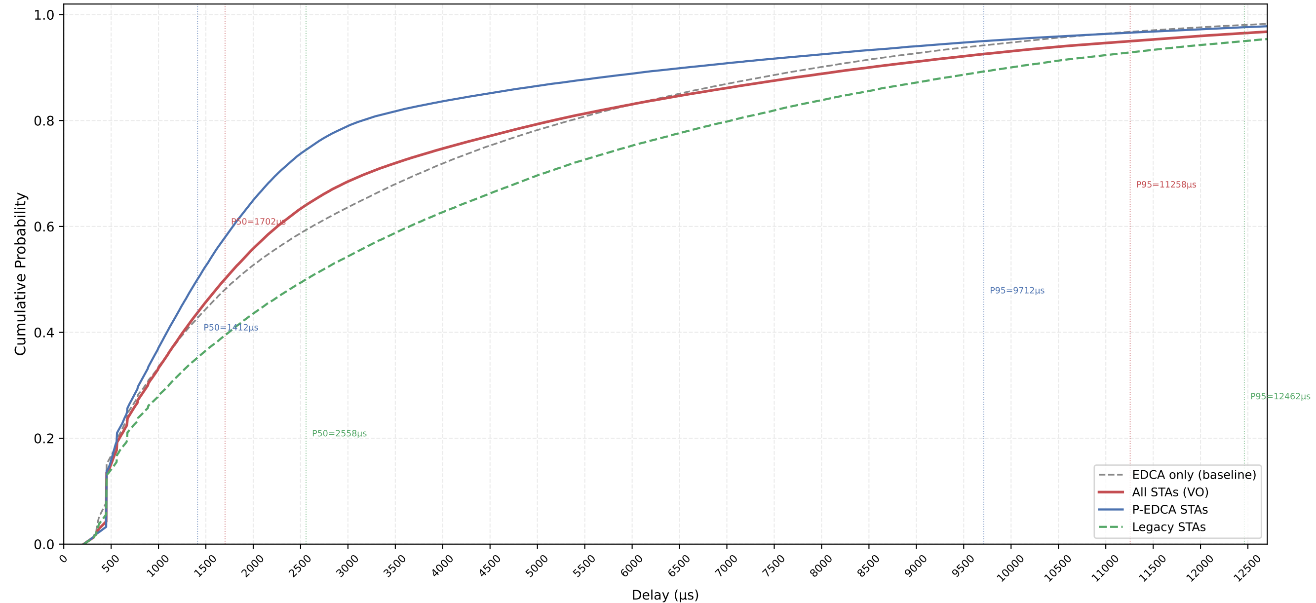
VO Delay CDF — P-EDCA / Legacy / All | CWds=0 × QSRC=0 × PSRC=2 nSta=30, nPedca=15/30, 1Mbps, avg of 10 runs
