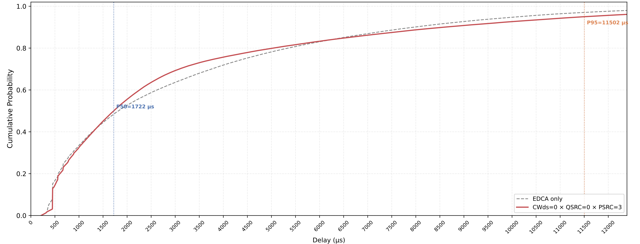
VO (all STAs) Delay CDF — CWds=0 × QSRC=0 × PSRC=3 nSta=30, nPedca=30, 1Mbps, avg of 10 runs
