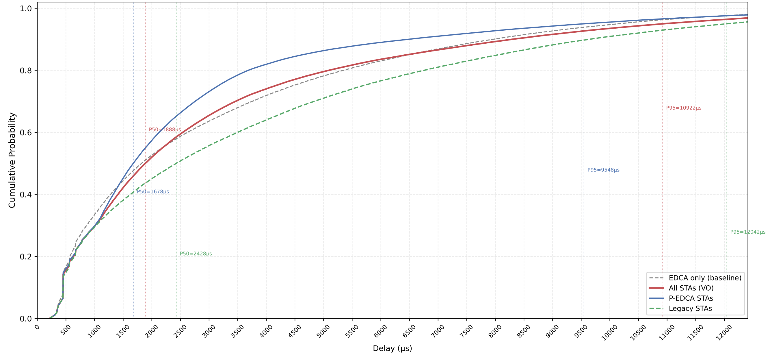
VO Delay CDF — P-EDCA / Legacy / All | CWds=0 × QSRC=1 × PSRC=3 nSta=30, nPedca=15/30, 1Mbps, avg of 10 runs
