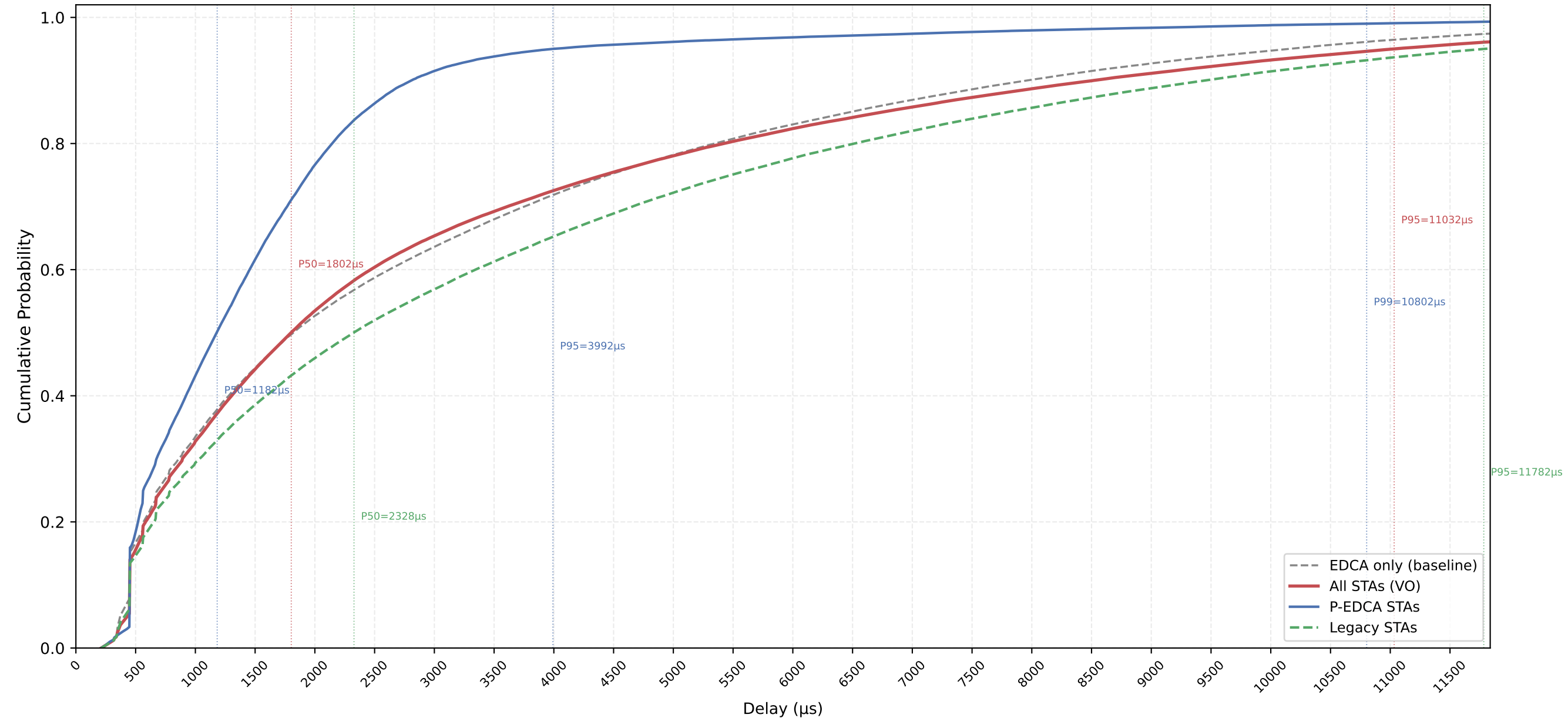
VO Delay CDF — P-EDCA / Legacy / All | CWds=1 × QSRC=0 × PSRC=3 nSta=30, nPedca=5/30, 1Mbps, avg of 10 runs
