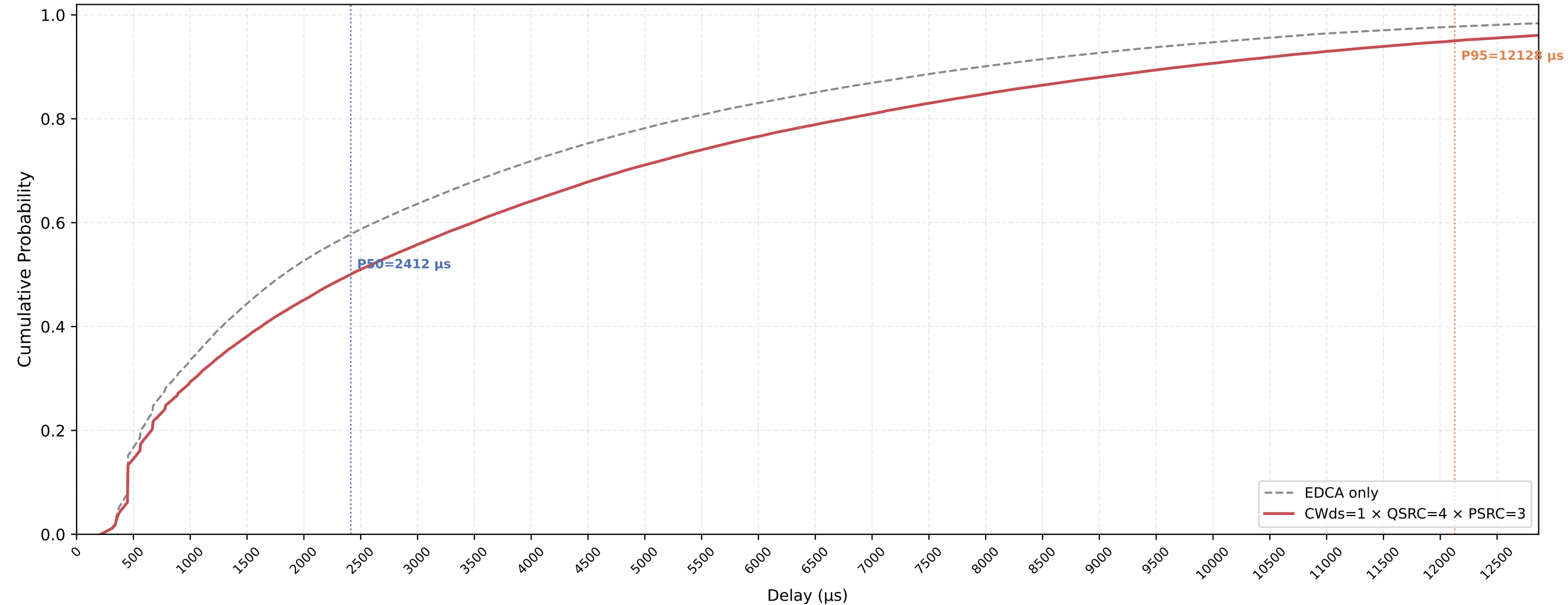
Legacy STA VO Delay CDF — CWds=1 × QSRC=4 × PSRC=3 nSta=30, nPedca=15, 1Mbps, avg of 10 runs
