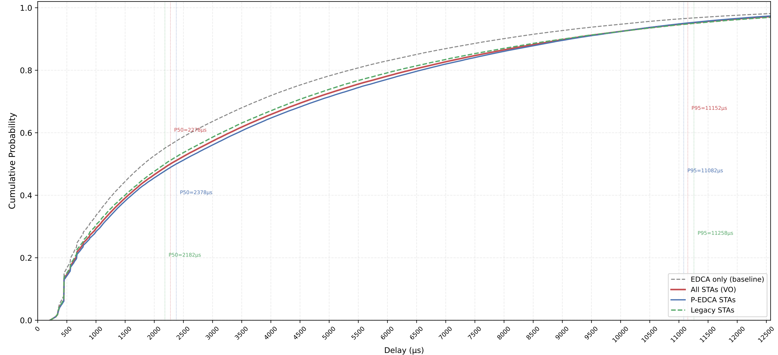
VO Delay CDF — P-EDCA / Legacy / All | CWds=1 × QSRC=5 × PSRC=1 nSta=30, nPedca=15/30, 1Mbps, avg of 10 runs
