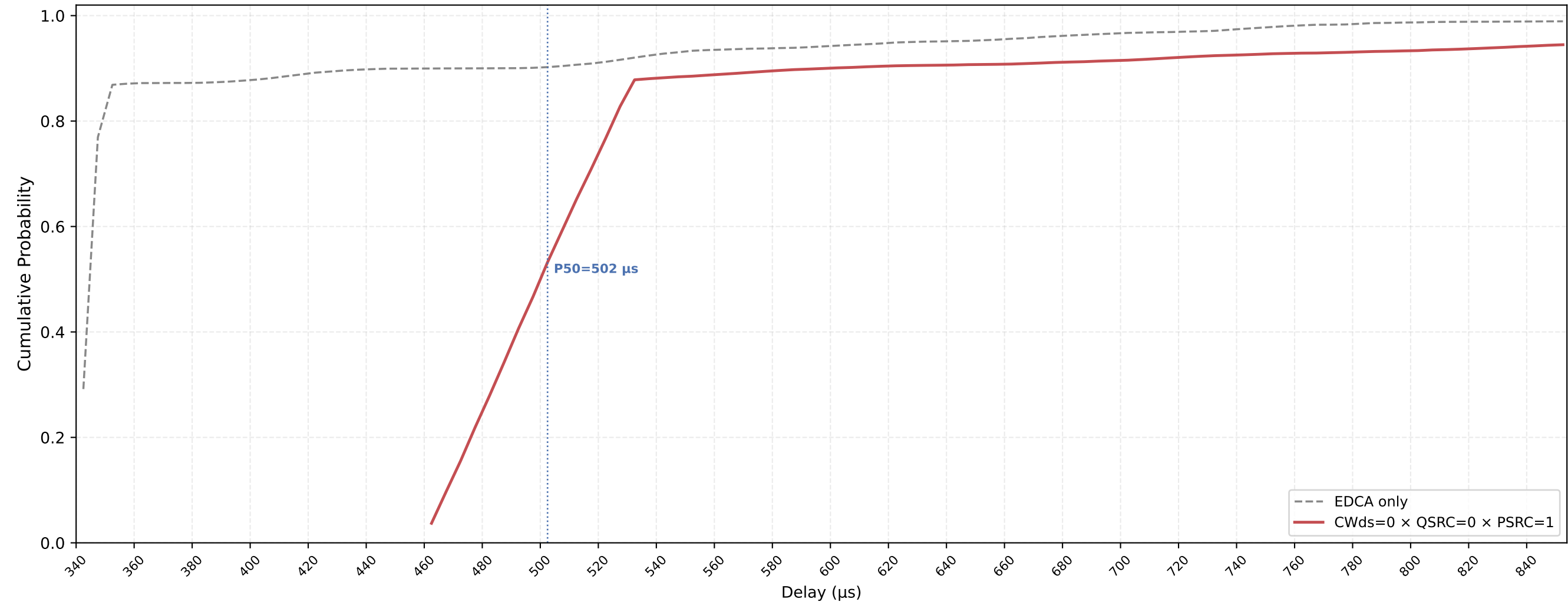
P-EDCA STA VO Delay CDF — CWds=0 × QSRC=0 × PSRC=1 nSta=30, nPedca=15, 0.1Mbps, avg of 10 runs
