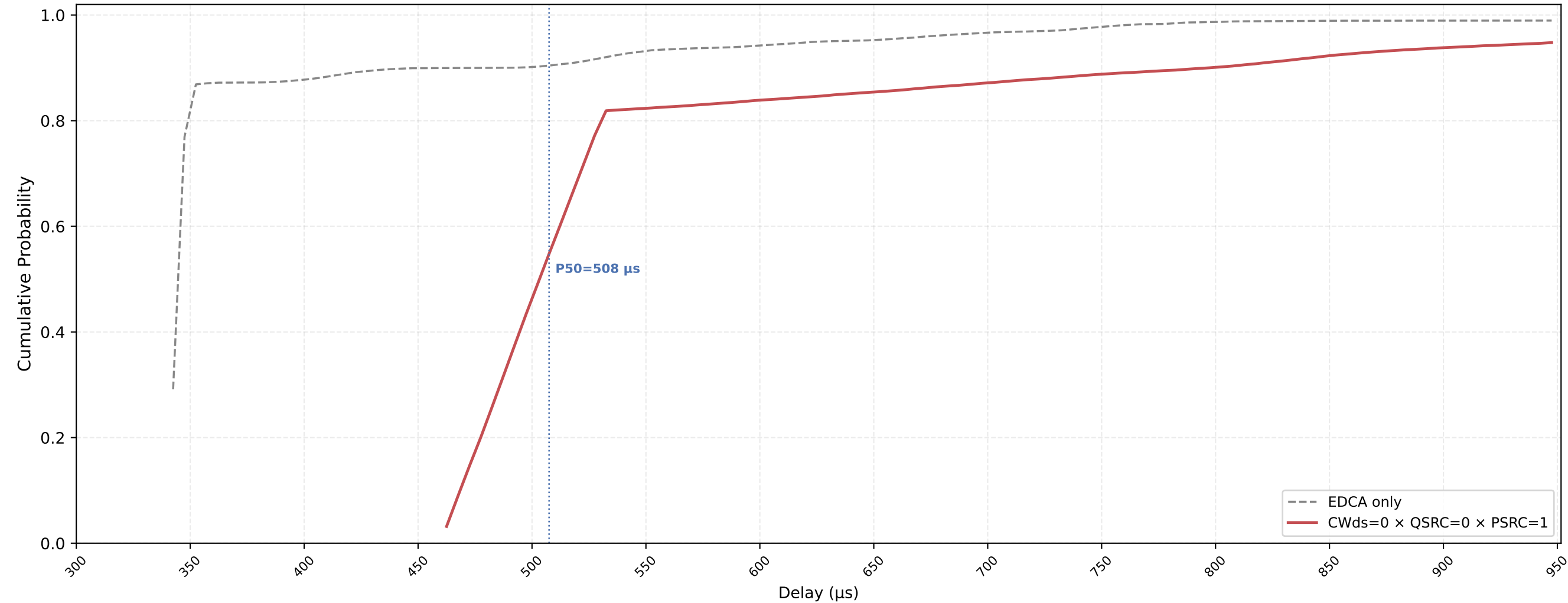
VO (all STAs) Delay CDF — CWds=0 × QSRC=0 × PSRC=1 nSta=30, nPedca=30, 0.1Mbps, avg of 10 runs
