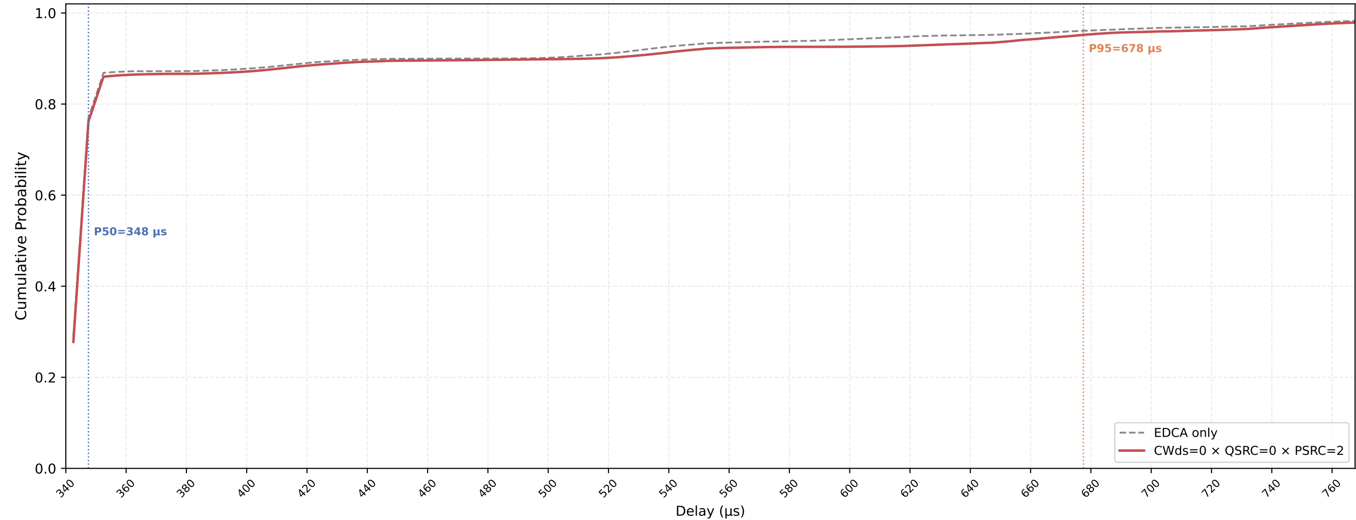
Legacy STA VO Delay CDF — CWds=0 × QSRC=0 × PSRC=2 nSta=30, nPedca=5, 0.1Mbps, avg of 10 runs
