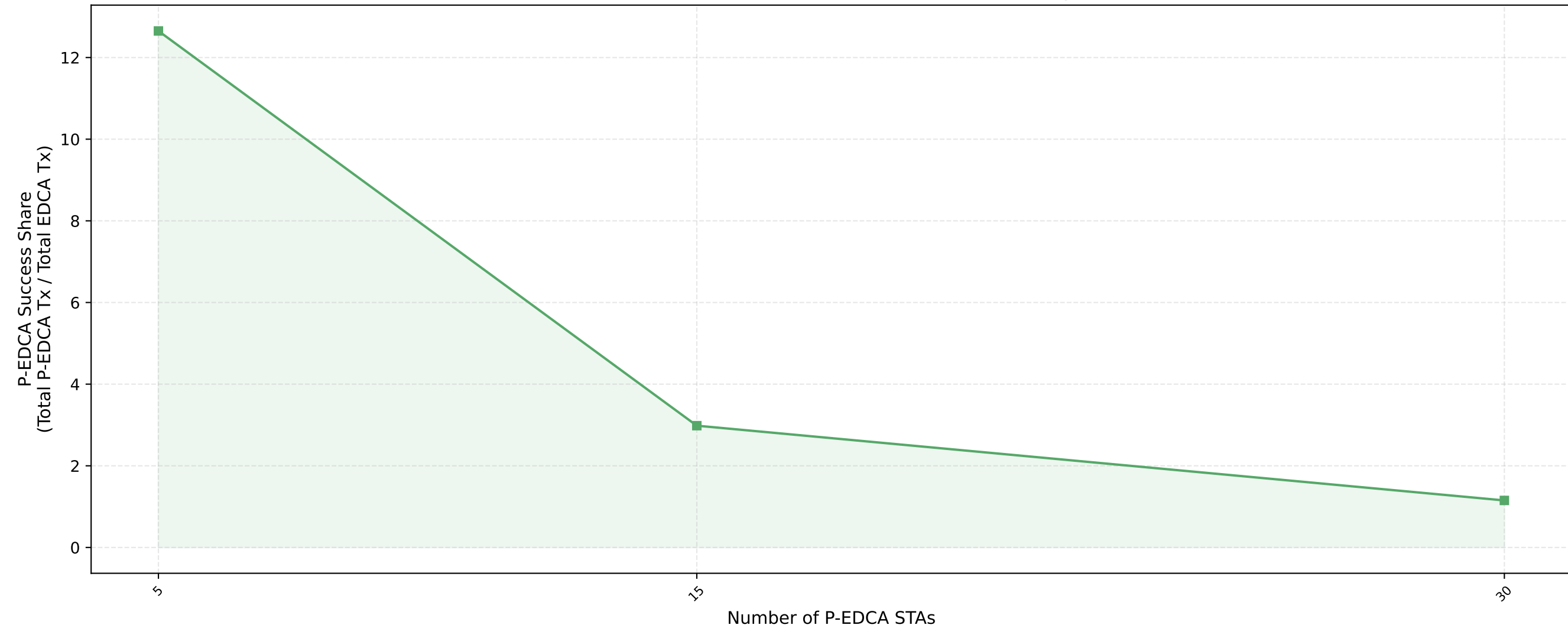
P-EDCA Tx / Total EDCA Tx — nSta=30, 0.5Mbps (avg of 10 runs)
