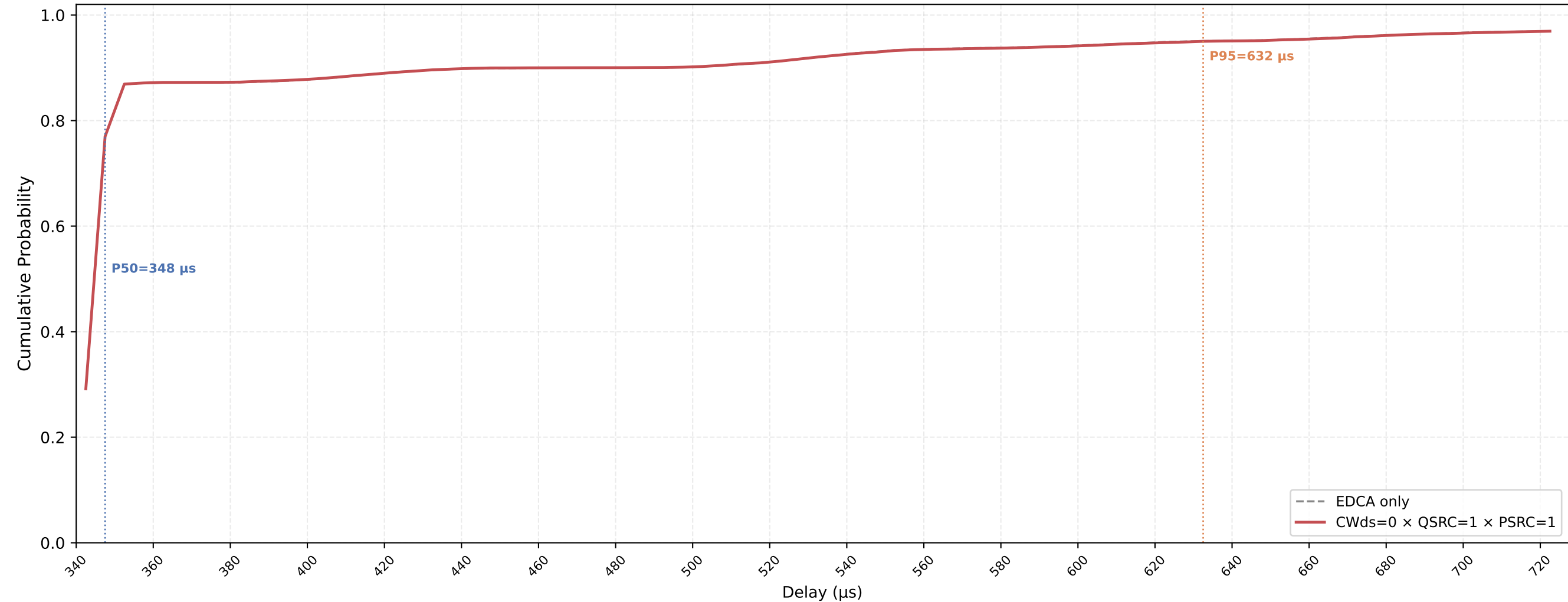
VO (all STAs) Delay CDF — CWds=0 × QSRC=1 × PSRC=1 nSta=30, nPedca=5, 0.1Mbps, avg of 10 runs
