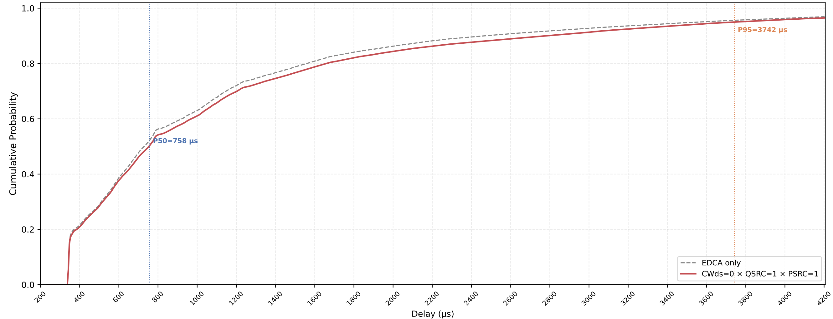
VO (all STAs) Delay CDF — CWds=0 × QSRC=1 × PSRC=1 nSta=30, nPedca=5, 0.5Mbps, avg of 10 runs
