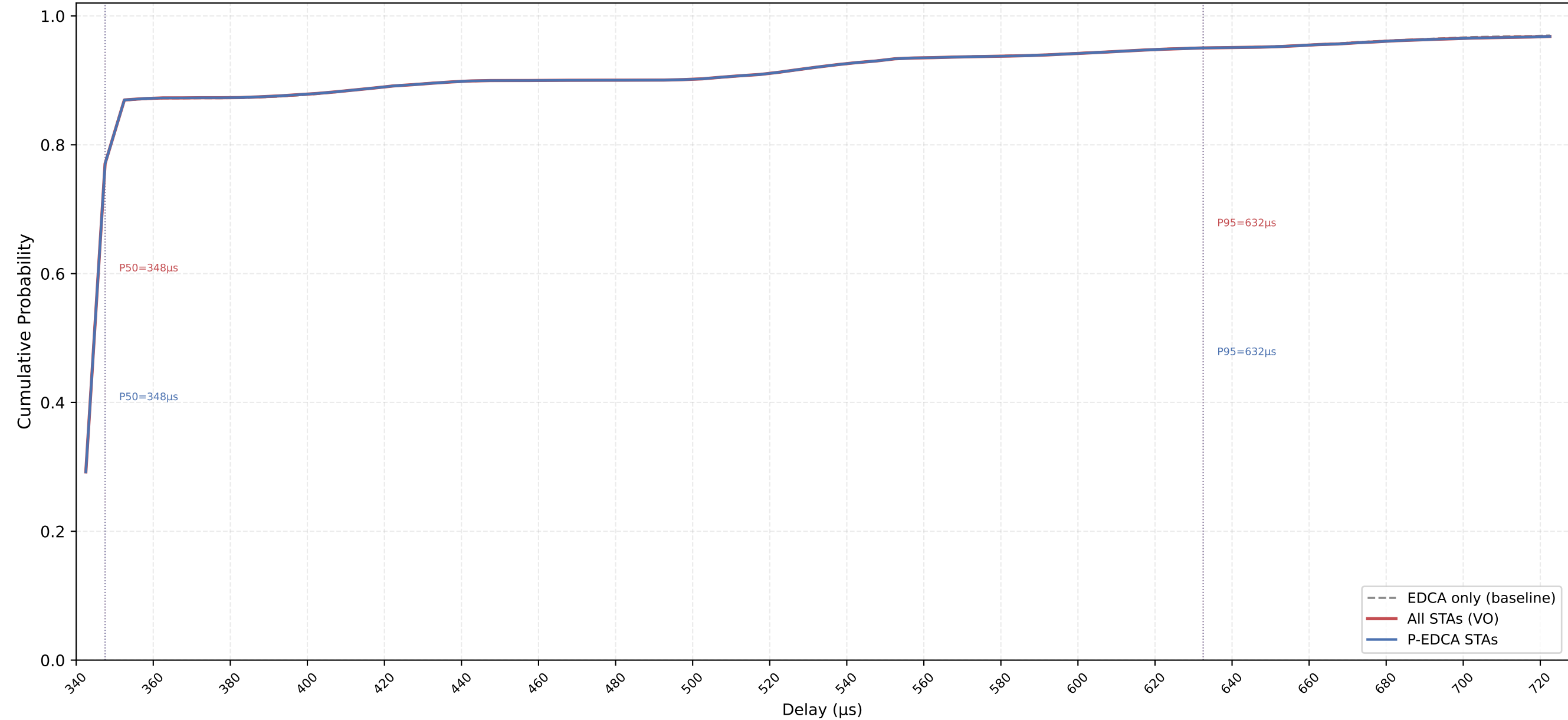
VO Delay CDF — P-EDCA / Legacy / All | CWds=0 × QSRC=1 × PSRC=2 nSta=30, nPedca=30/30, 0.1Mbps, avg of 10 runs
