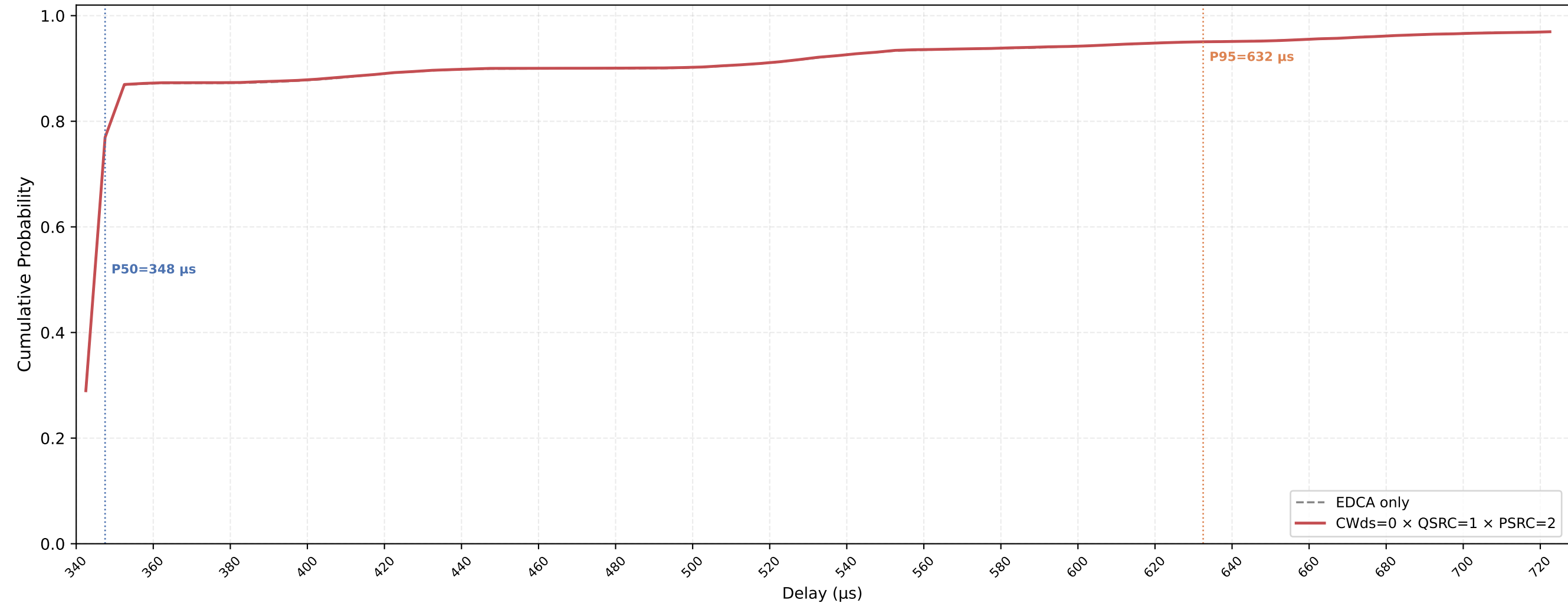
VO (all STAs) Delay CDF — CWds=0 × QSRC=1 × PSRC=2 nSta=30, nPedca=5, 0.1Mbps, avg of 10 runs
