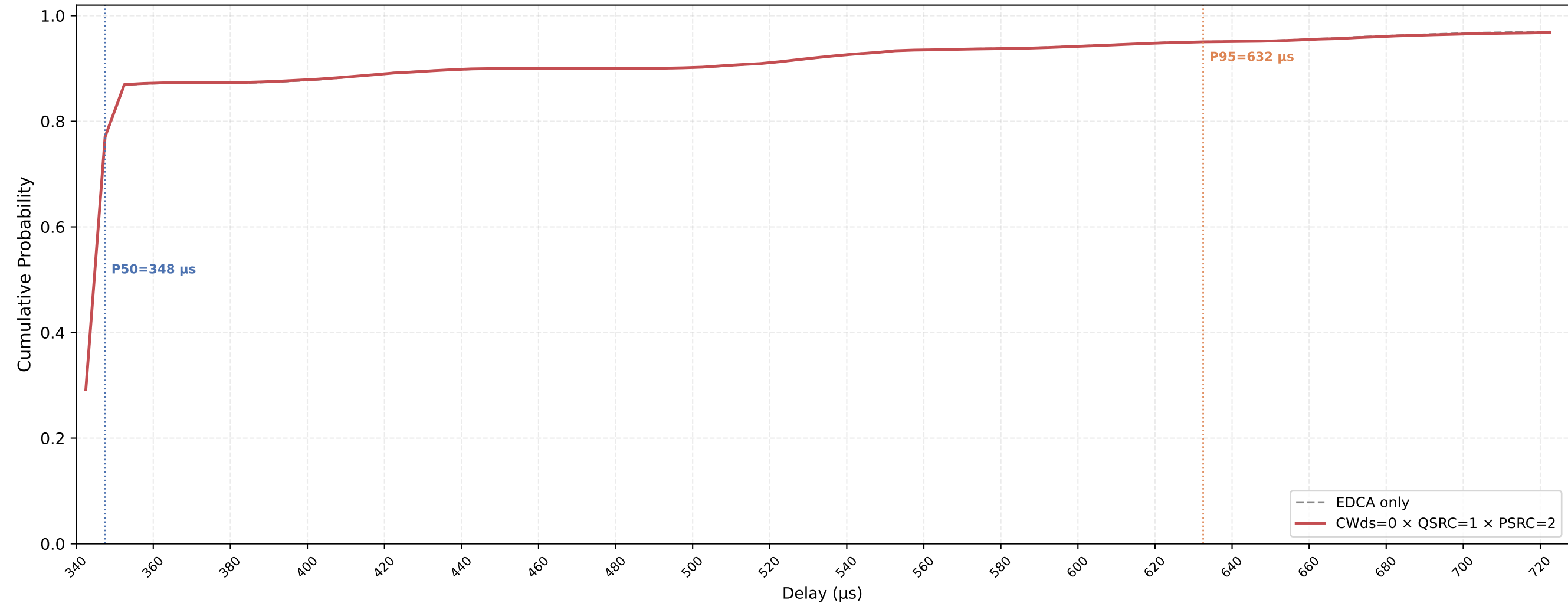
VO (all STAs) Delay CDF — CWds=0 × QSRC=1 × PSRC=2 nSta=30, nPedca=30, 0.1Mbps, avg of 10 runs
