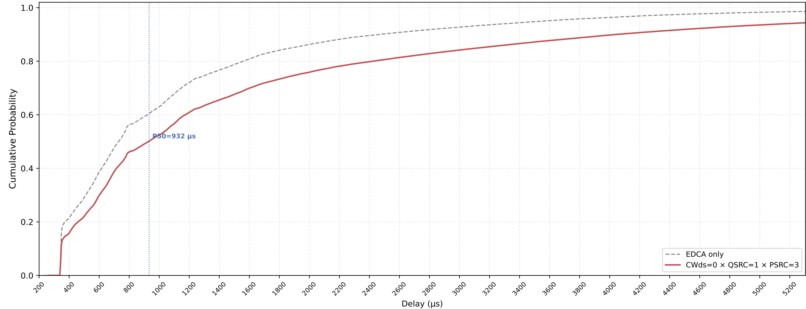
Legacy STA VO Delay CDF — CWds=0 × QSRC=1 × PSRC=3 nSta=30, nPedca=15, 0.5Mbps, avg of 10 runs
