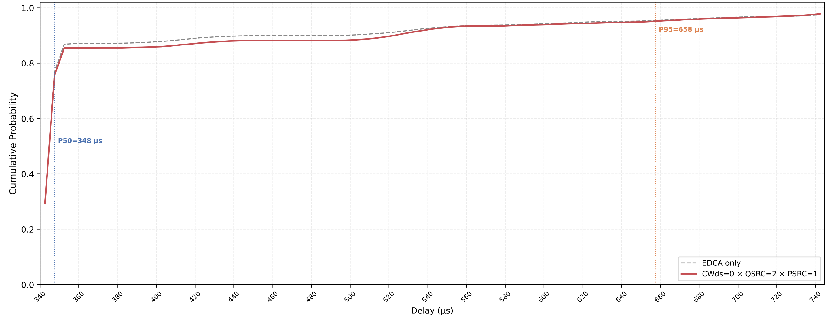
Legacy STA VO Delay CDF — CWds=0 × QSRC=2 × PSRC=1 nSta=30, nPedca=15, 0.1Mbps, avg of 10 runs
