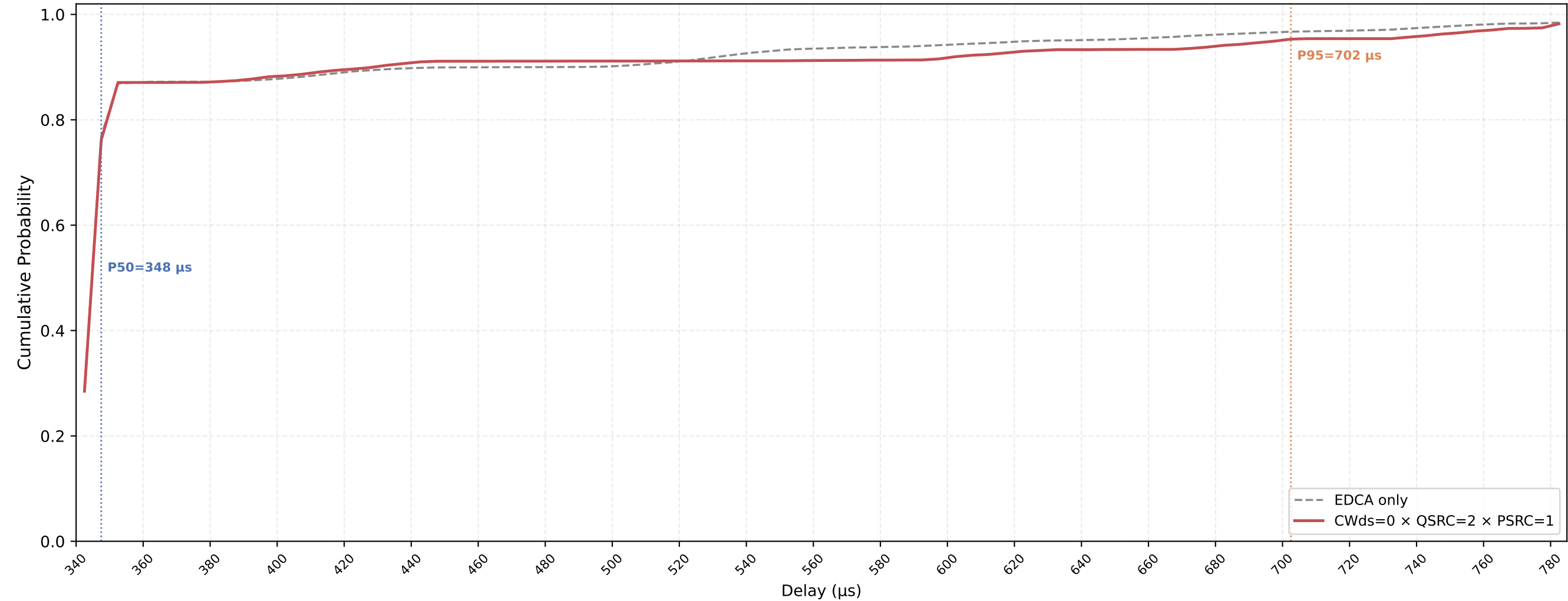
P-EDCA STA VO Delay CDF — CWds=0 × QSRC=2 × PSRC=1 nSta=30, nPedca=5, 0.1Mbps, avg of 10 runs
