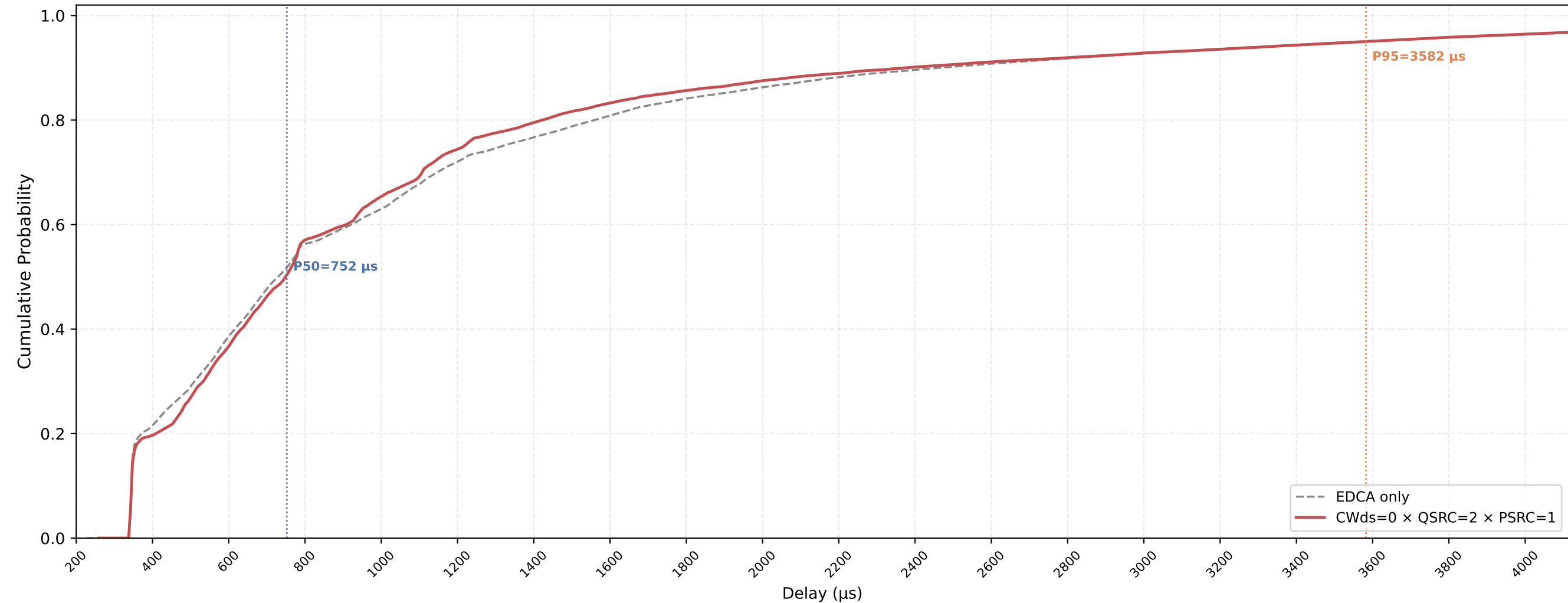
P-EDCA STA VO Delay CDF — CWds=0 × QSRC=2 × PSRC=1 nSta=30, nPedca=5, 0.5Mbps, avg of 10 runs
