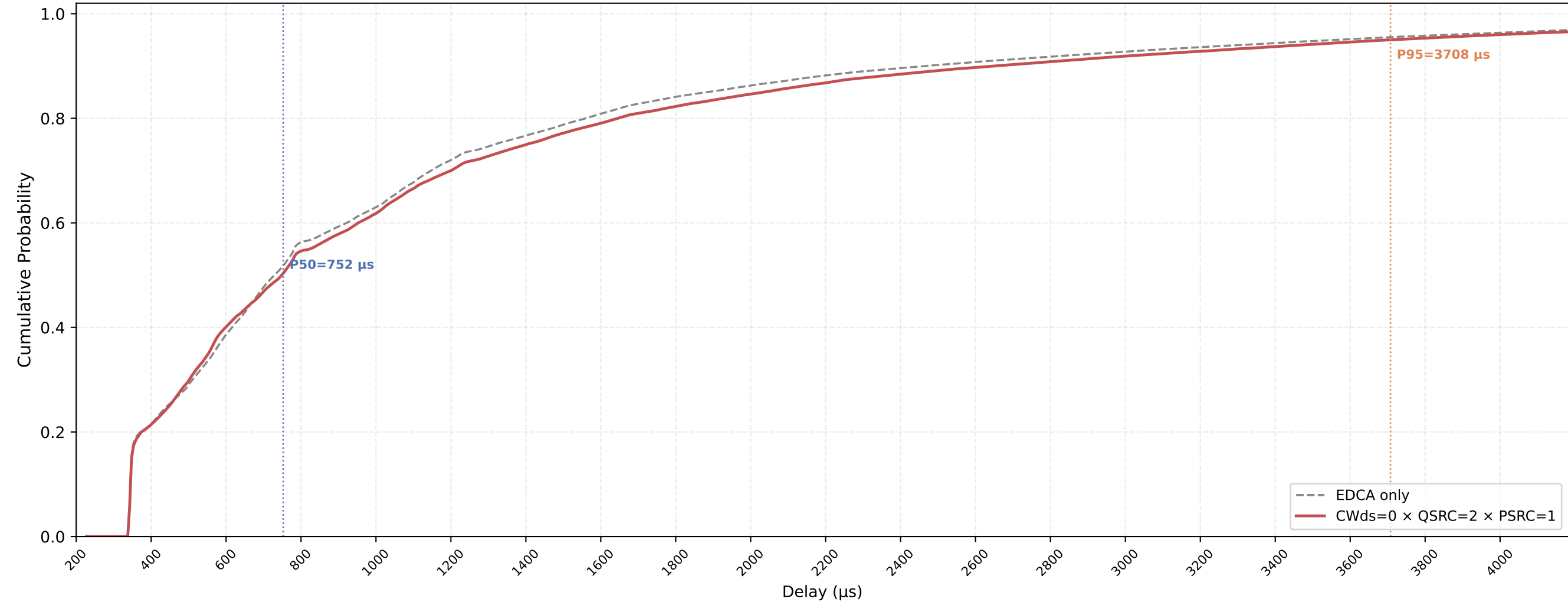
P-EDCA STA VO Delay CDF — CWds=0 × QSRC=2 × PSRC=1 nSta=30, nPedca=15, 0.5Mbps, avg of 10 runs
