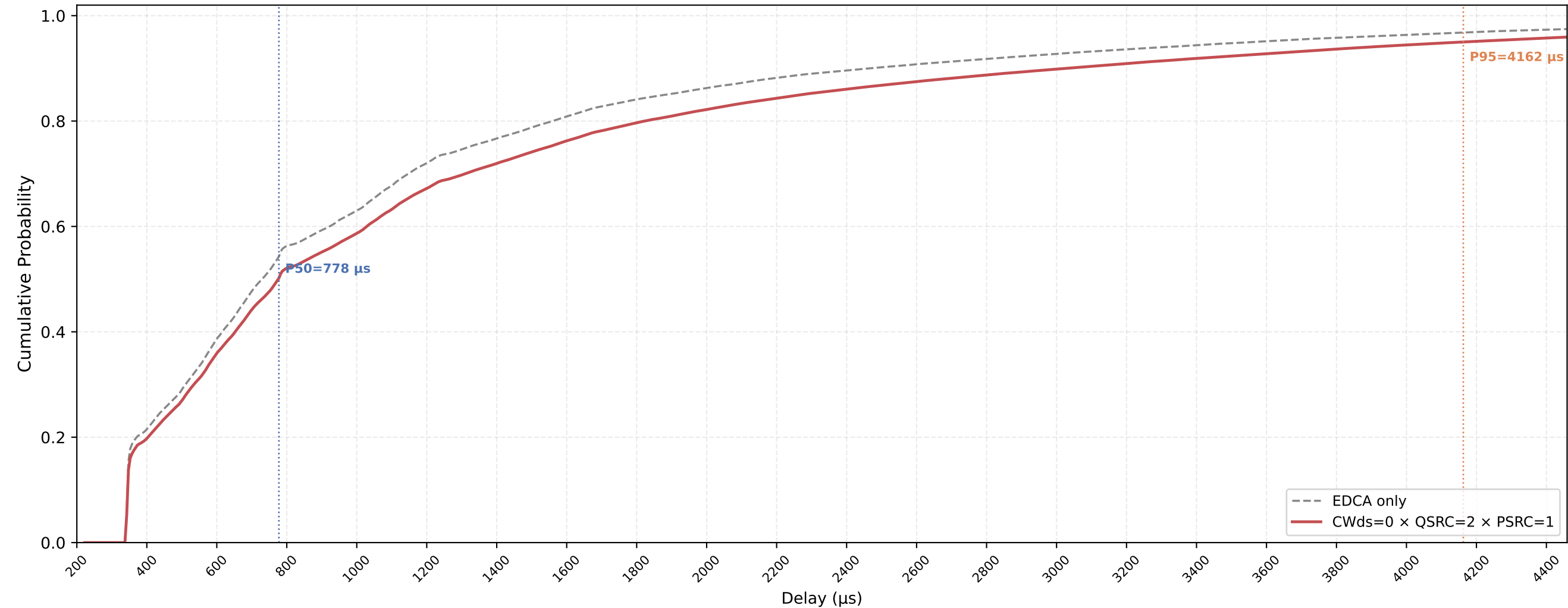
P-EDCA STA VO Delay CDF — CWds=0 × QSRC=2 × PSRC=1 nSta=30, nPedca=30, 0.5Mbps, avg of 10 runs
