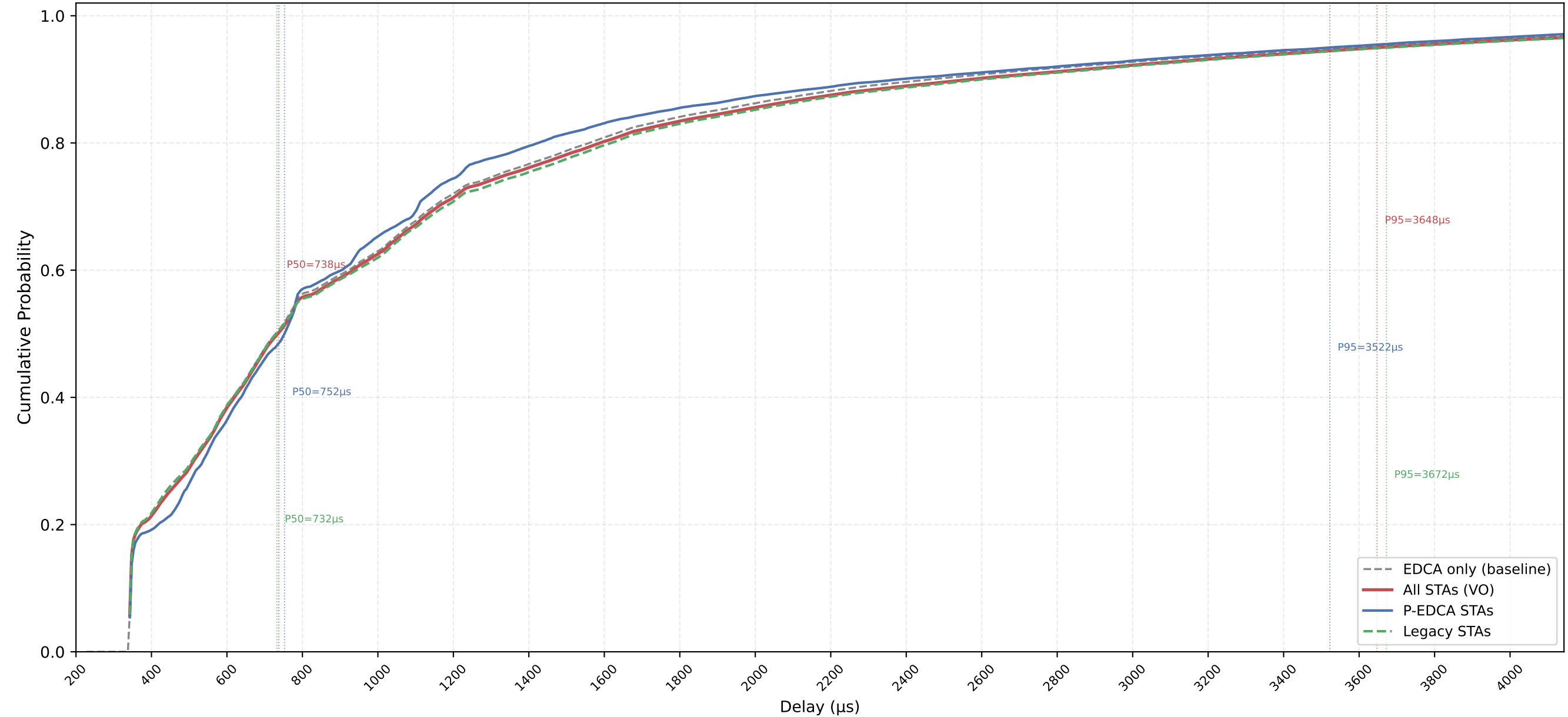
VO Delay CDF — P-EDCA / Legacy / All | CWds=0 × QSRC=2 × PSRC=2 nSta=30, nPedca=5/30, 0.5Mbps, avg of 10 runs
