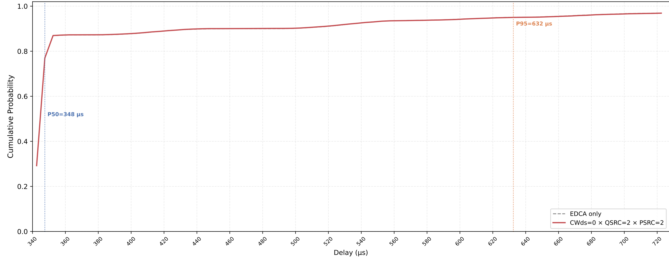
P-EDCA STA VO Delay CDF — CWds=0 × QSRC=2 × PSRC=2 nSta=30, nPedca=30, 0.1Mbps, avg of 10 runs
