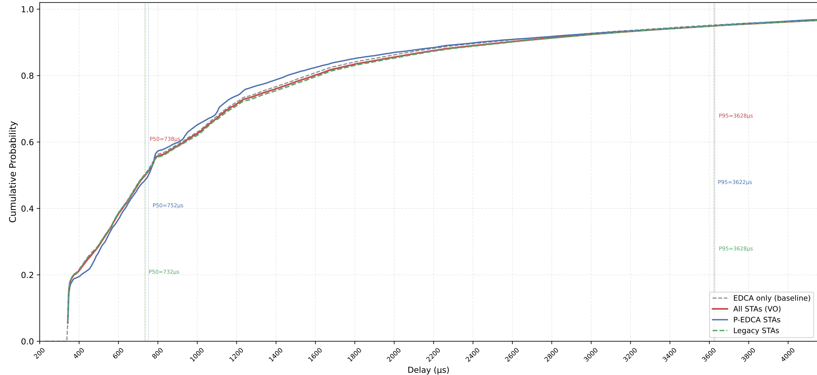
VO Delay CDF — P-EDCA / Legacy / All | CWds=0 × QSRC=2 × PSRC=3 nSta=30, nPedca=5/30, 0.5Mbps, avg of 10 runs
