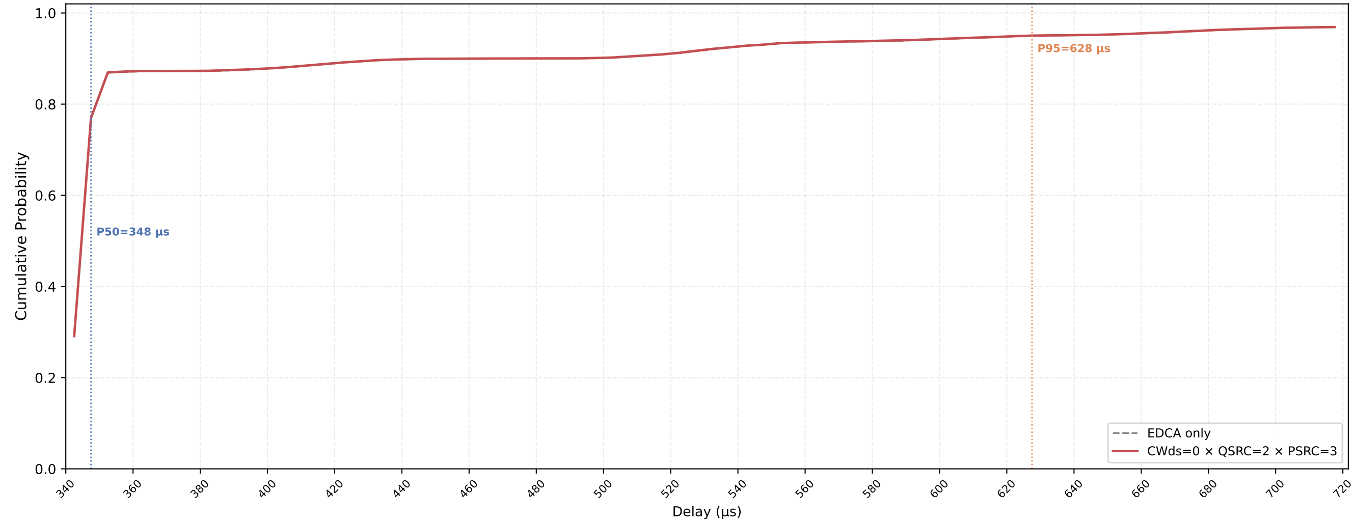
VO (all STAs) Delay CDF — CWds=0 × QSRC=2 × PSRC=3 nSta=30, nPedca=15, 0.1Mbps, avg of 10 runs
