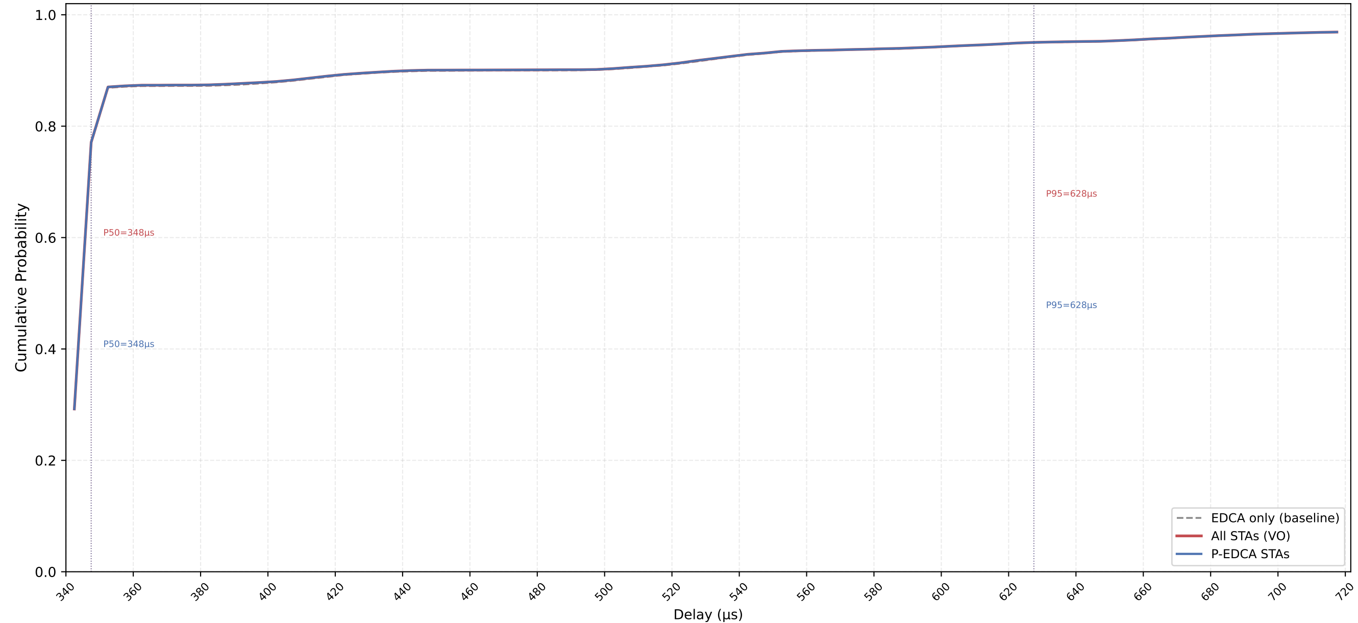
VO Delay CDF — P-EDCA / Legacy / All | CWds=0 × QSRC=4 × PSRC=1 nSta=30, nPedca=30/30, 0.1Mbps, avg of 10 runs
