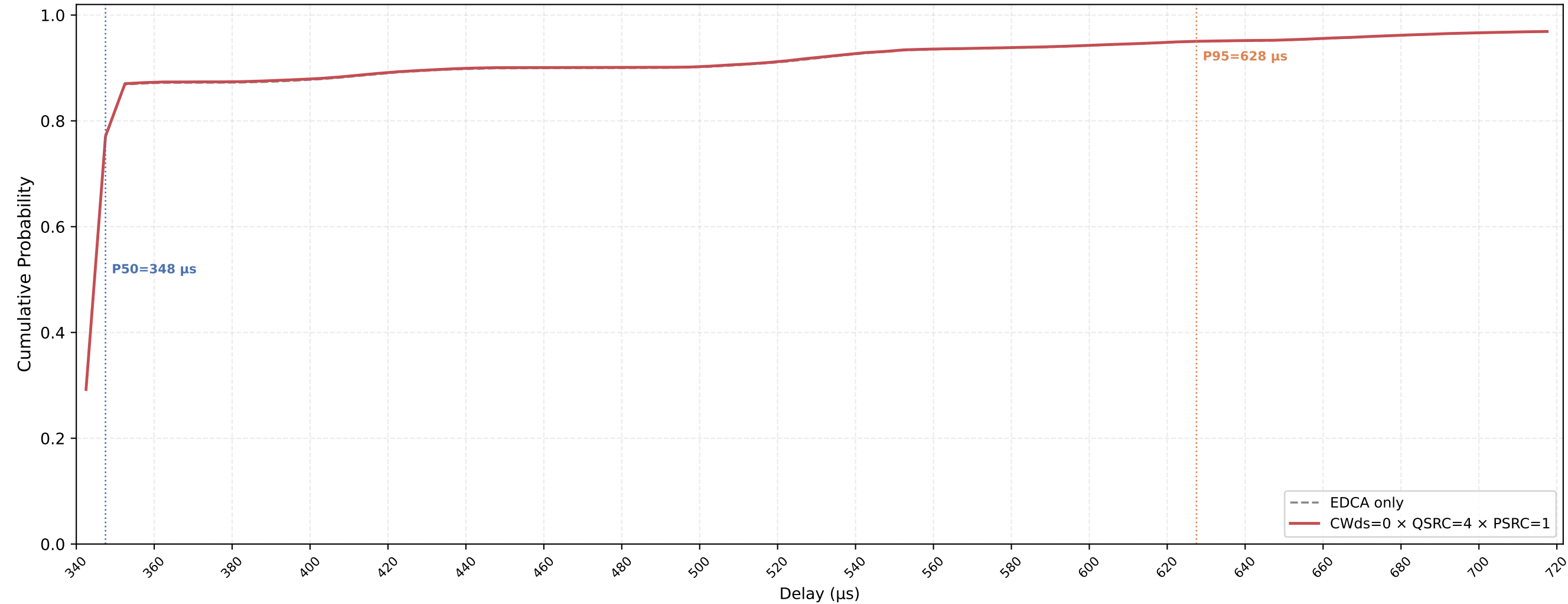
P-EDCA STA VO Delay CDF — CWds=0 × QSRC=4 × PSRC=1 nSta=30, nPedca=30, 0.1Mbps, avg of 10 runs
