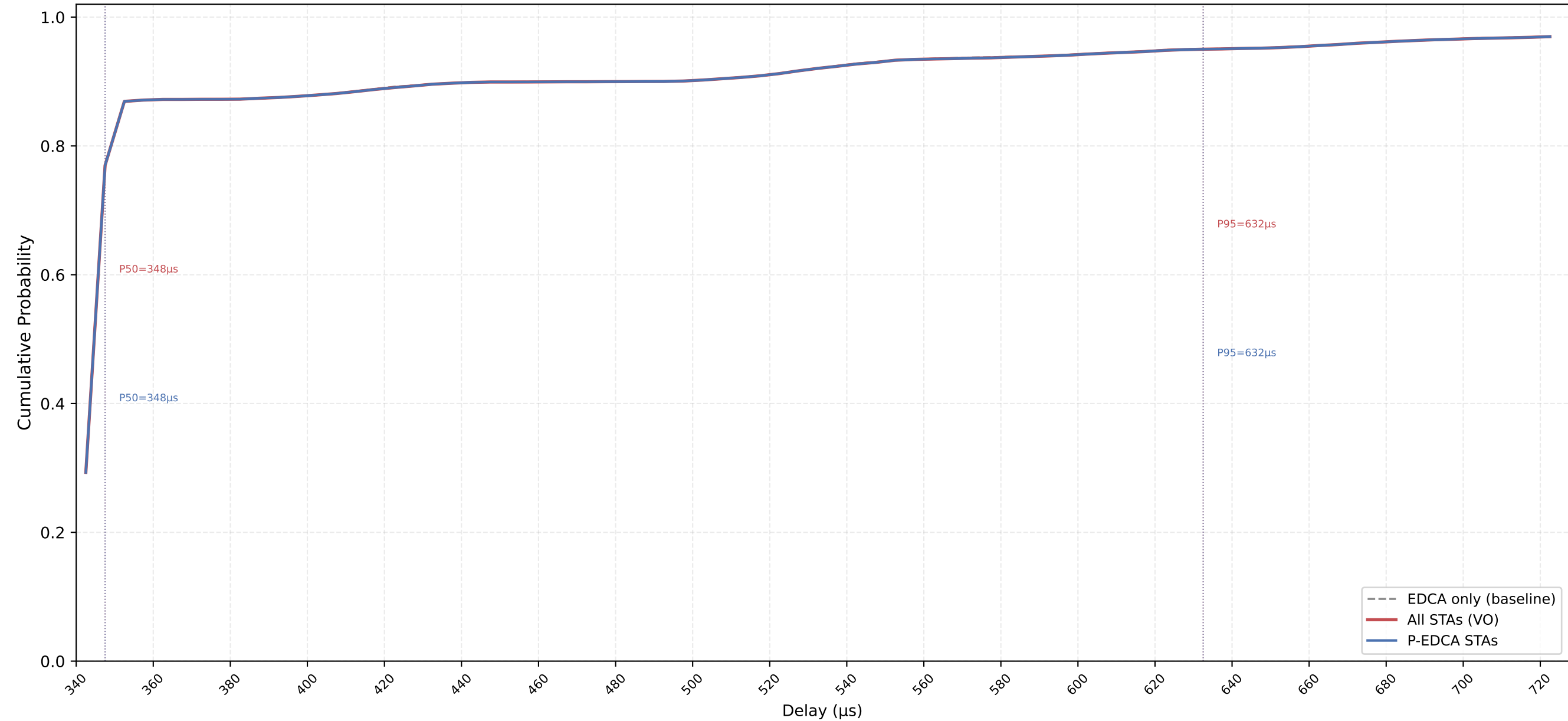
VO Delay CDF — P-EDCA / Legacy / All | CWds=0 × QSRC=4 × PSRC=2 nSta=30, nPedca=30/30, 0.1Mbps, avg of 10 runs
