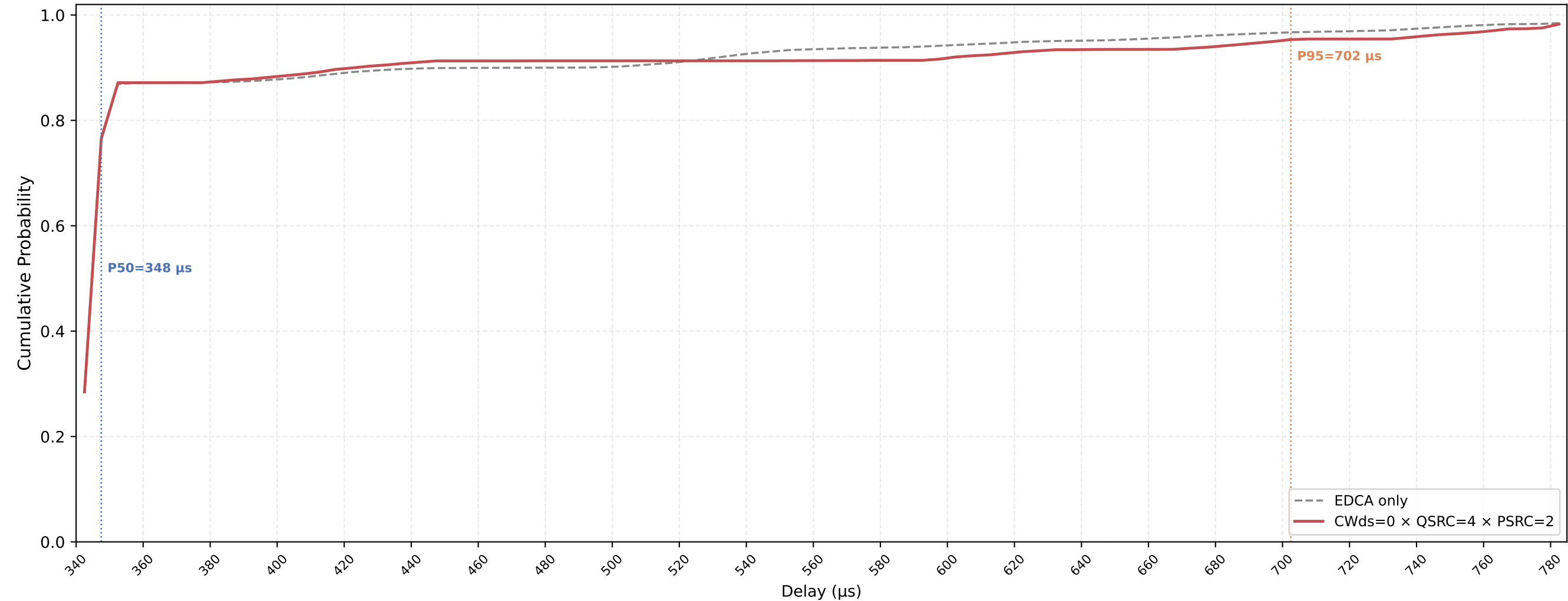
P-EDCA STA VO Delay CDF — CWds=0 × QSRC=4 × PSRC=2 nSta=30, nPedca=5, 0.1Mbps, avg of 10 runs
