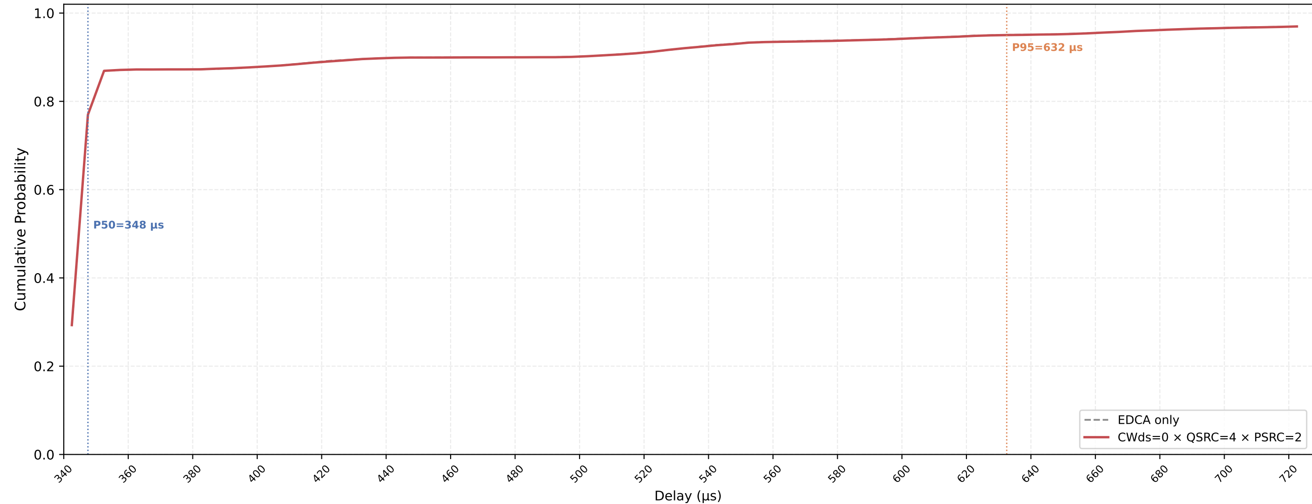
P-EDCA STA VO Delay CDF — CWds=0 × QSRC=4 × PSRC=2 nSta=30, nPedca=30, 0.1Mbps, avg of 10 runs
