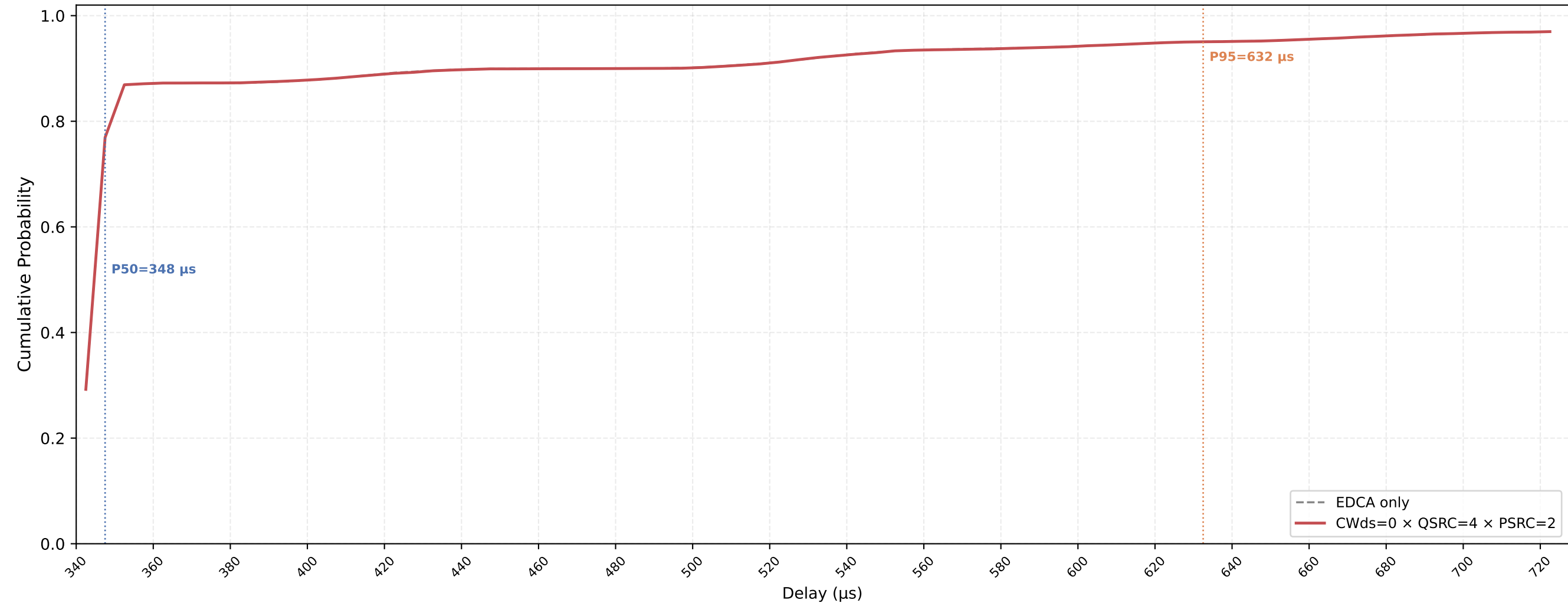
VO (all STAs) Delay CDF — CWds=0 × QSRC=4 × PSRC=2 nSta=30, nPedca=15, 0.1Mbps, avg of 10 runs
