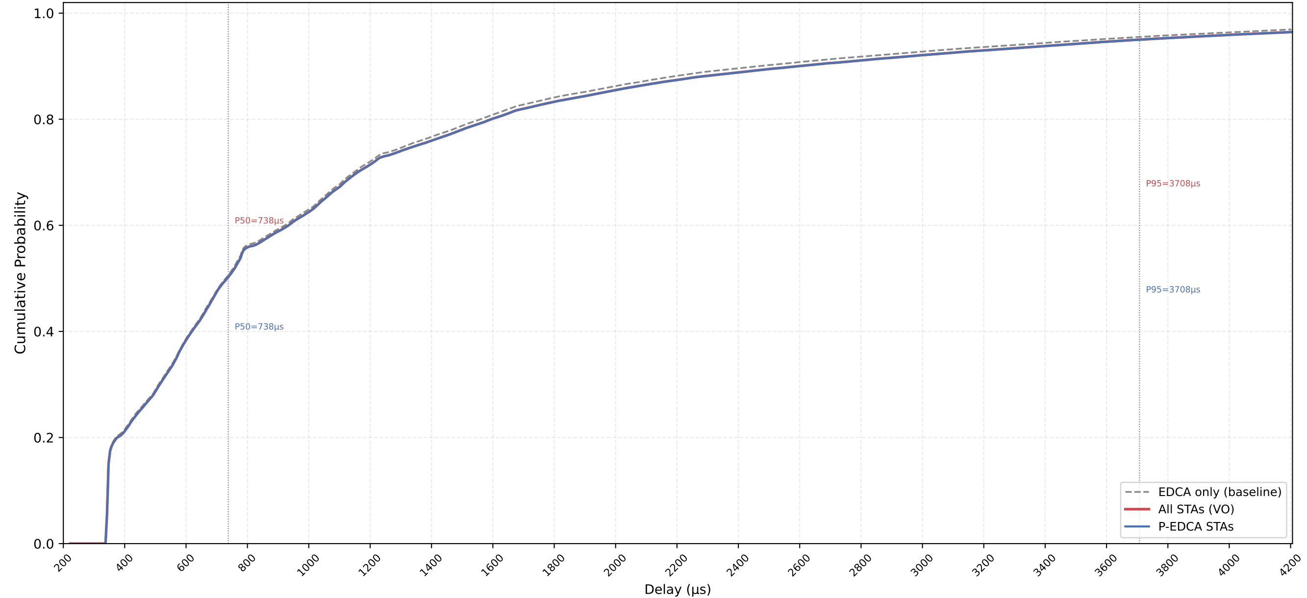
VO Delay CDF — P-EDCA / Legacy / All | CWds=0 × QSRC=4 × PSRC=3 nSta=30, nPedca=30/30, 0.5Mbps, avg of 10 runs
