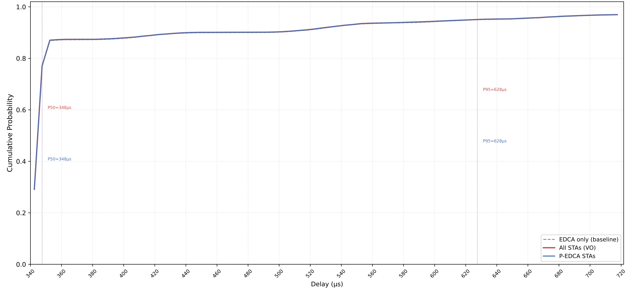
VO Delay CDF — P-EDCA / Legacy / All | CWds=0 × QSRC=5 × PSRC=1 nSta=30, nPedca=30/30, 0.1Mbps, avg of 10 runs
