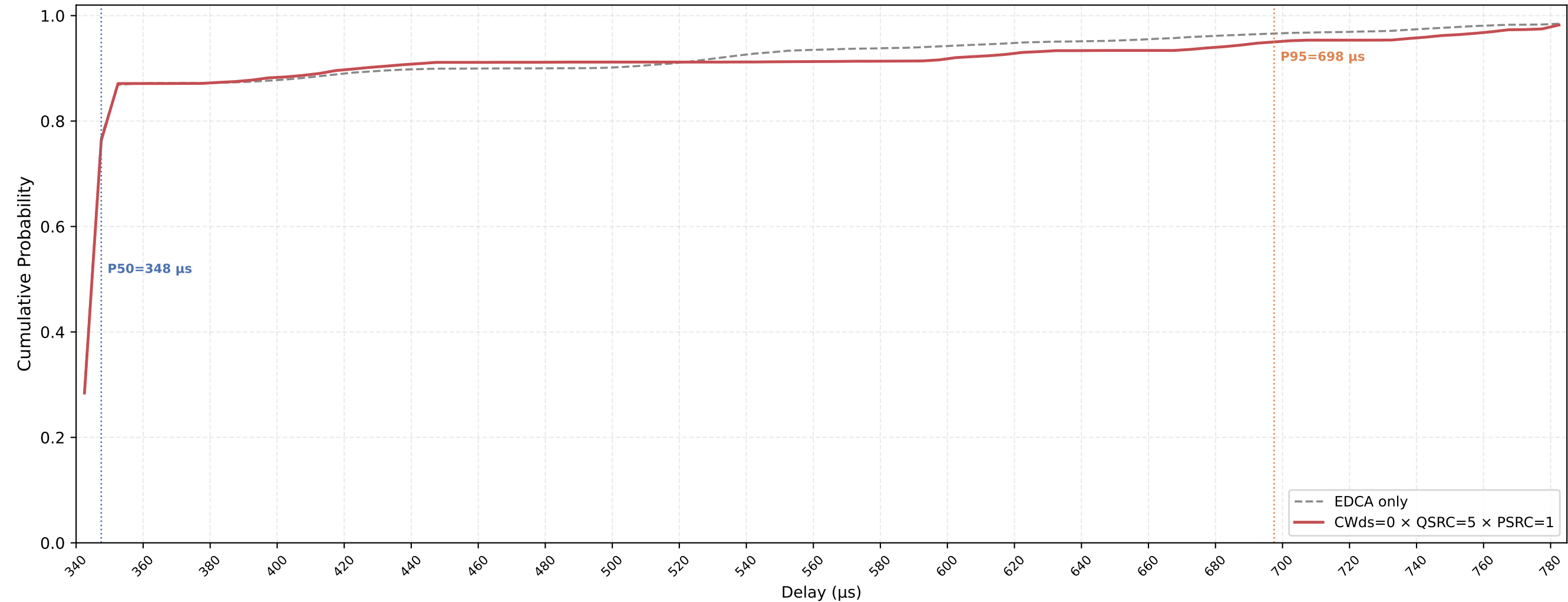
P-EDCA STA VO Delay CDF — CWds=0 × QSRC=5 × PSRC=1 nSta=30, nPedca=5, 0.1Mbps, avg of 10 runs
