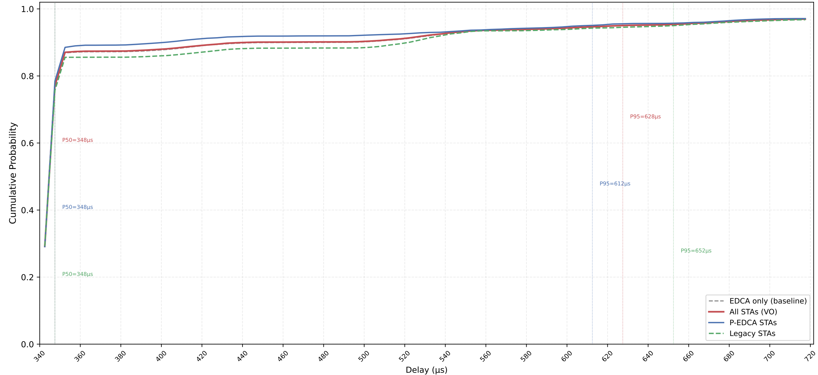
VO Delay CDF — P-EDCA / Legacy / All | CWds=0 × QSRC=5 × PSRC=3 nSta=30, nPedca=15/30, 0.1Mbps, avg of 10 runs
